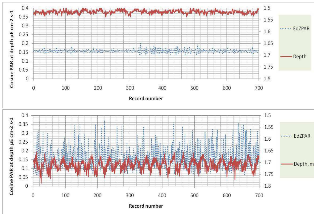
Fig. 4. PAR fluctuations as measured by PRR800 at 0.8 m depth: A) on a very calm day (0.4 m/sec wind); and B) on a windy day (7 m/sec wind). The depth values are not calibrated but do represent the amplitude of surface waves as sensed by the pressure sensor of the PRR800 unit. Data were recorded at 15 Hz without any shading effect, downwind of the IUI pier, in the gulf of Eilat. Coefficient of variance=40% (Dishon, personal communication)
