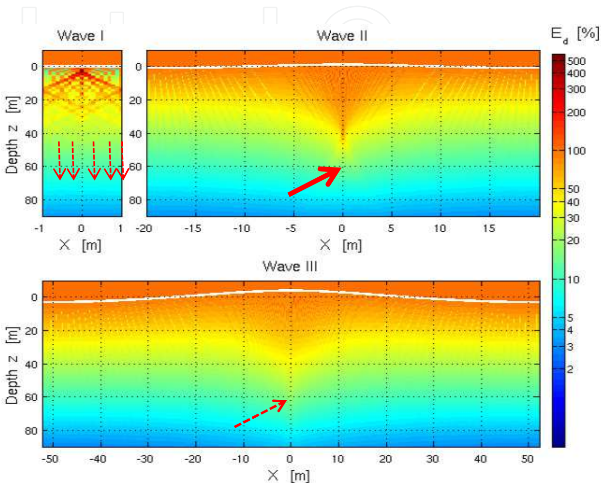
Fig. 3. Downward irradiance patterns below three waves with respect to 100% at the surface (note the logarithmic color scale and the different scales of the x axes) Wave I, flat surface, no lensing; Wave II, strong lensing; wave III, large radius, weak lensing (after Hieronymi and Macke (2010)).
