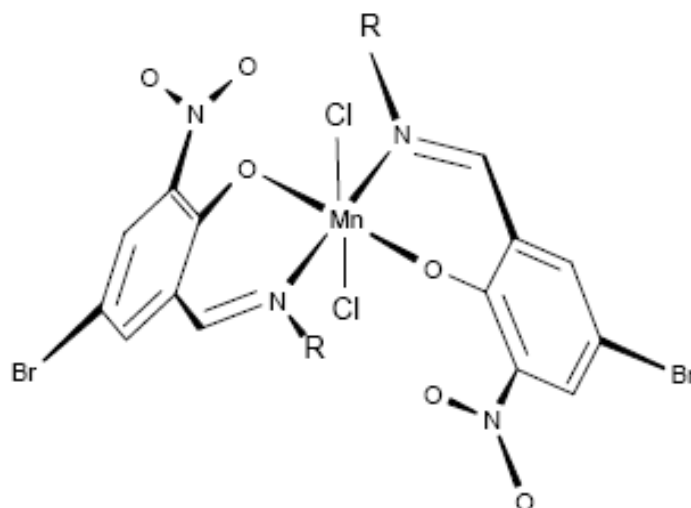
Fig. 9. Structure of the complex \text{trans-Mn(IV)L}_2\text{Cl}_2 ( \text{L} = \text{N-alkyl-3-nitrosalicylidene} ) (Fujiwara et al., 1985).
