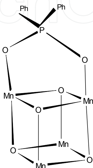
Fig. 11. Synthetic complexes \text{Mn}_4\text{O}_4(\text{O}_2\text{PR}_2)_6 , R = Ph and 4-MePh (only one \text{O}_2\text{PR}_2 is shown).
