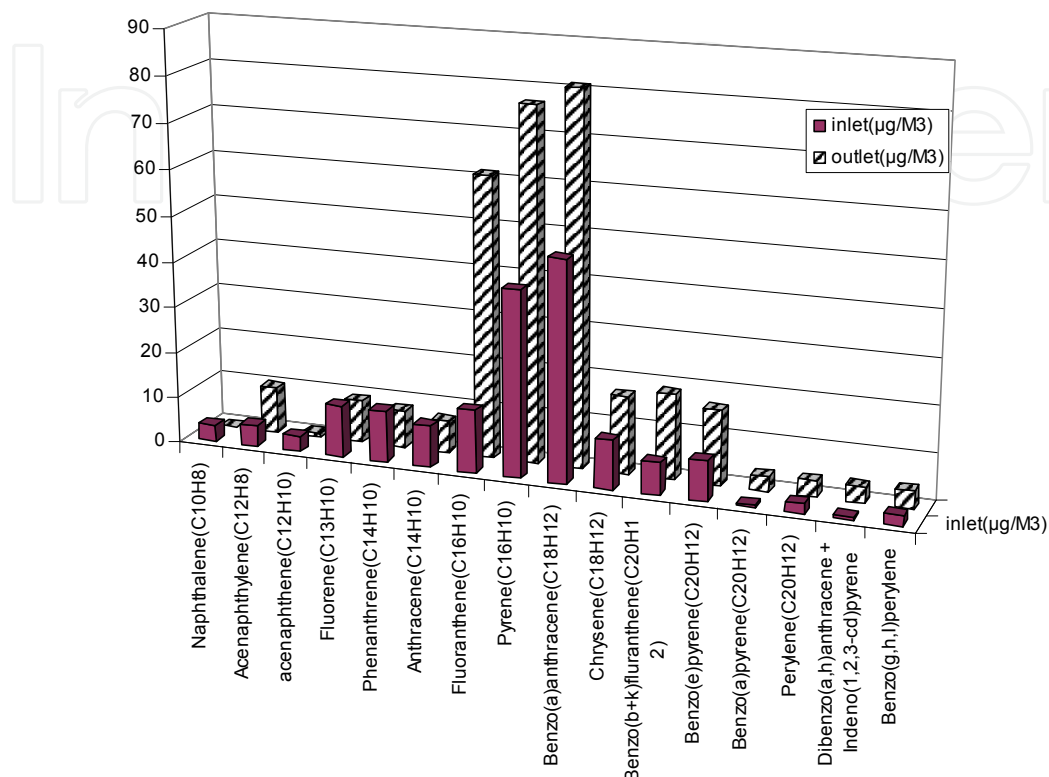
Fig. 7. EB irradiation influence on PAHs removal.
