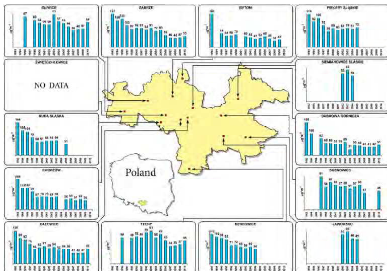
Fig. 2. The PM 10 concentrations ( \mu\text{g m}^{-3} ) in 14 cities of the Silesian Agglomeration in 1993-2010 (SSI, 1980-2006; The Provincial Inspector for Environmental Protection in Katowice [PIEP], 2002-2011)
