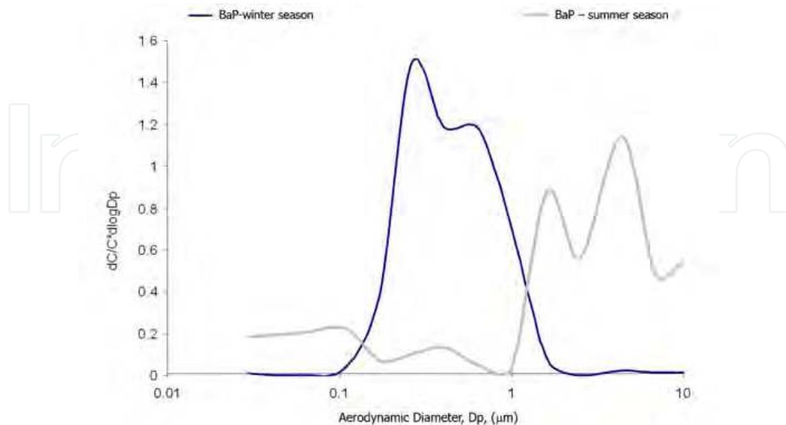
Fig. 10. Mass size distribution of PM-bound BaP relative to the aerodynamic diameter of the particles BaP is adsorbed on in Zabrze in winter and summer 2007
