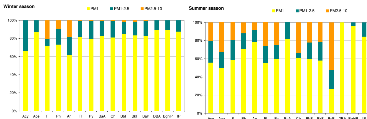
Fig. 6. Contribution of PM_1 -, PM_{1-2.5} - and PM_{2.5-10} -bound PAH to PM_{10} -bound PAH in Zabrze in winter and summer 2007
