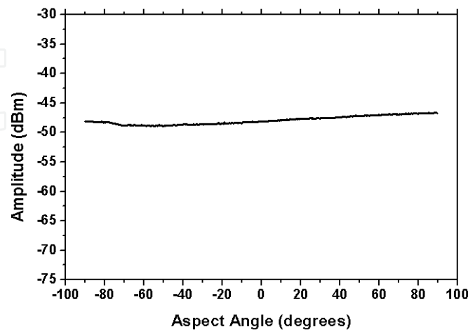
Fig. 18. RCS pattern of a cylinder at 9.375 GHz.
