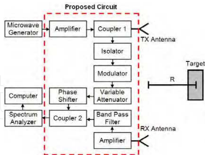
Fig. 5. Block diagram of the measurement system with the active noise cancellation circuit.
