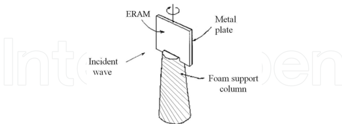
Fig. 10. Device scheme used for the RCS measurements.
