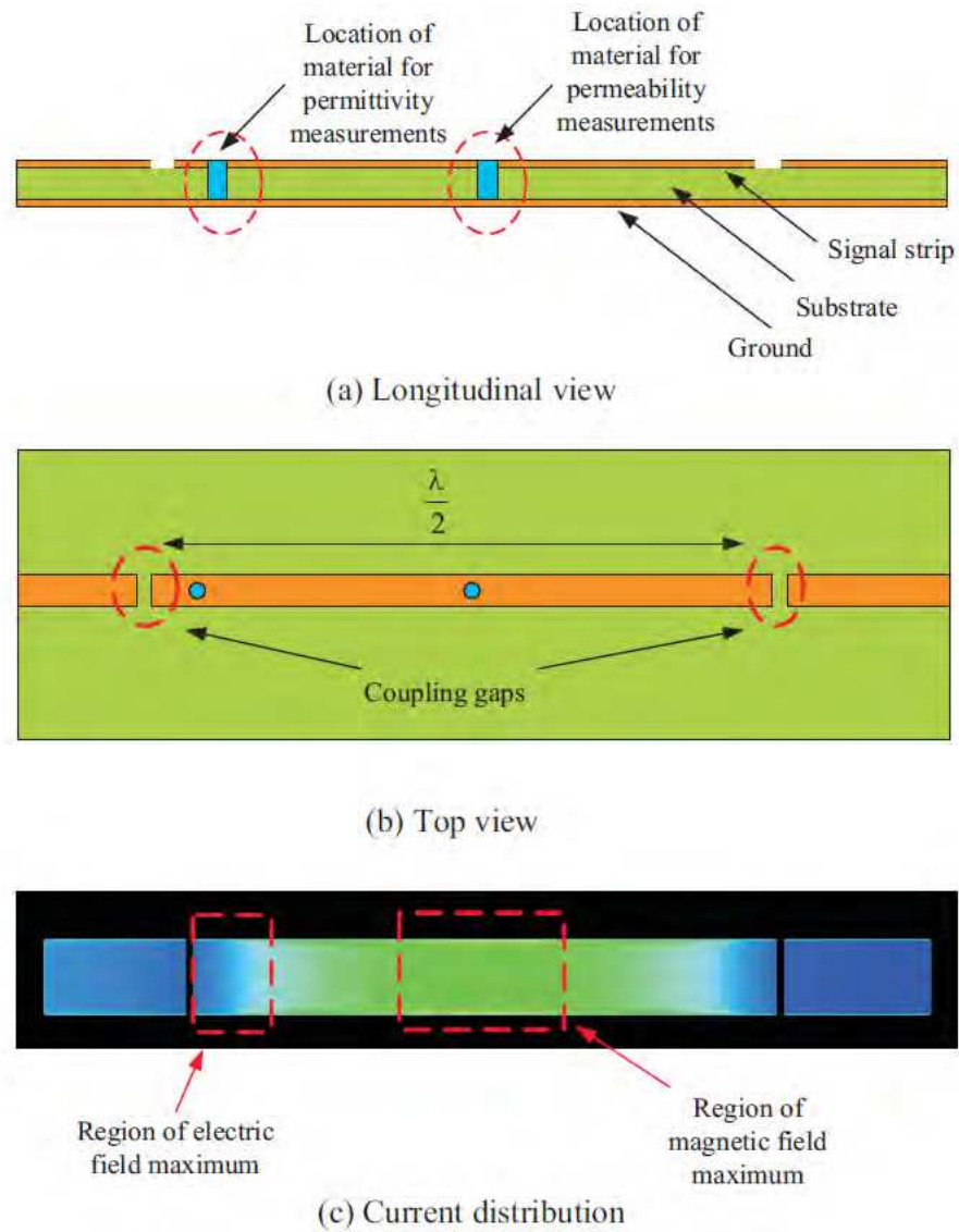
Fig. 10. Microstrip fixture for resonant perturbation measurements on liquid samples.
