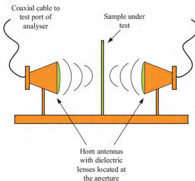
Fig. 2. Typical arrangement of a free space dielectric measurement setup.
