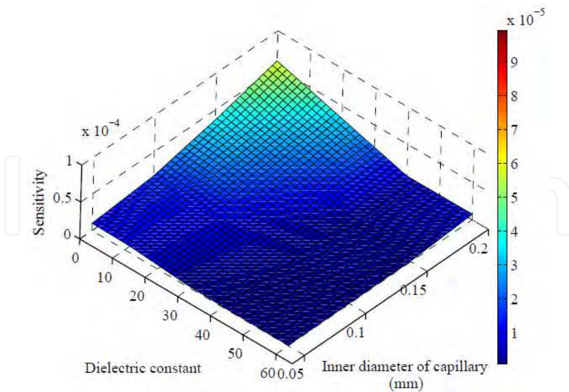
Fig. 23. Sensitivity versus the dielectric constant of material under test with varying inner diameter of capillary (Outer diameter of capillary = 0.7 mm).
