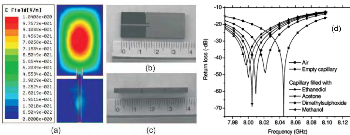
Fig. 25. (a) Magnitude of electric field distribution on the substrate integrated waveguide resonator for the fundamental TE_{101} resonant mode; (b) Top view of fabricated resonator; (c) Side view of fabricated resonator; (d) Measured return loss performance of various solvents.
