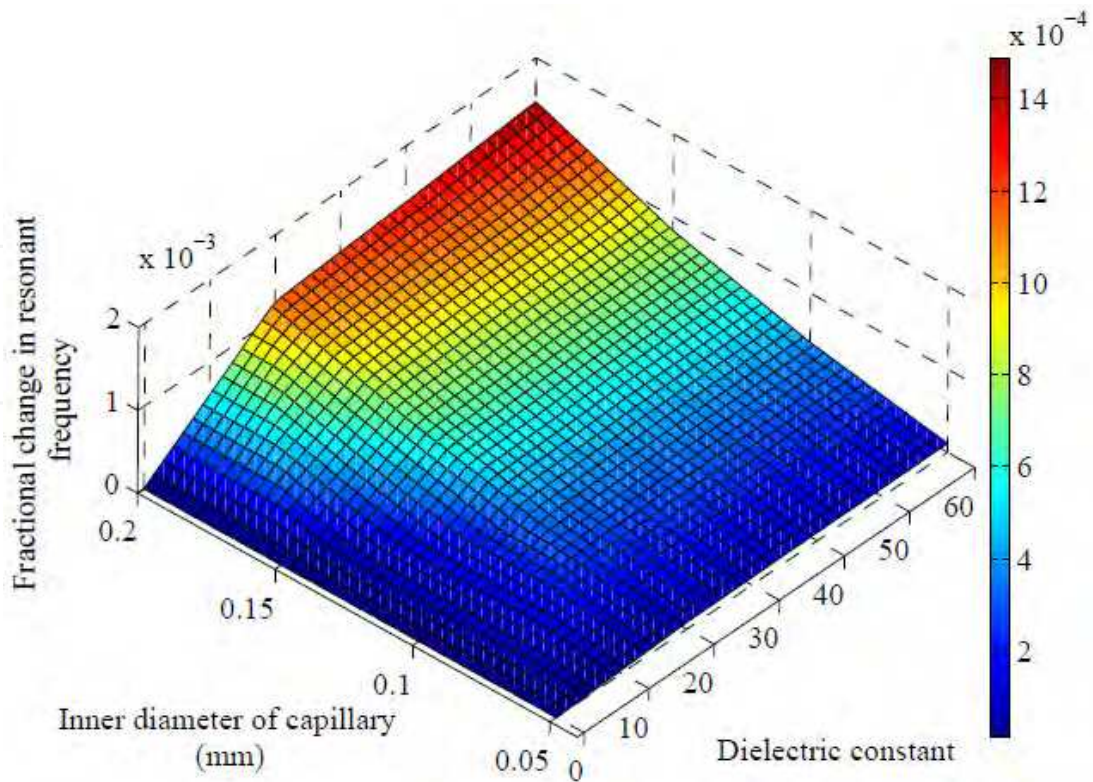
Fig. 22. Fractional change in resonant frequency with varying dielectric constant of an ideal lossless material for different inner diameters of capillary (Outer diameter of capillary = 0.7 mm).
