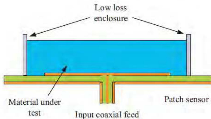
Fig. 11. Patch resonator sensor for complex permittivity measurements.
