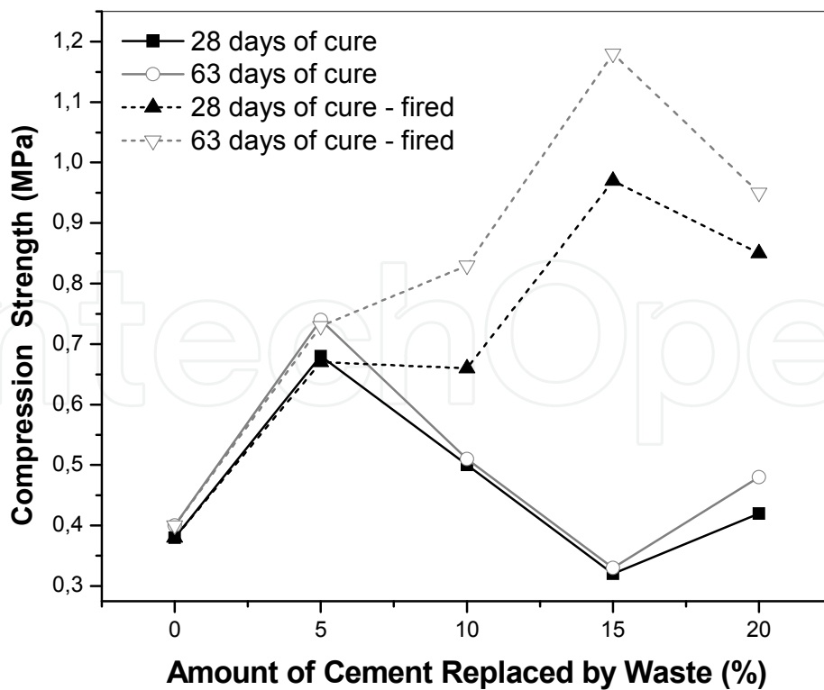
Fig. 11. Compression strength of mortar (cement:sand), which had part of the cement replaced by kaolin processing waste
