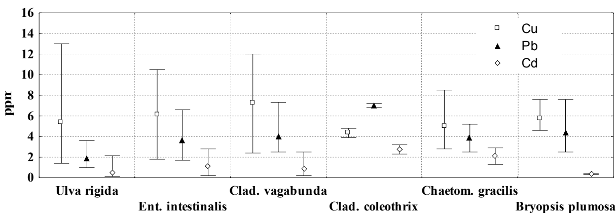
Fig. 14. Mean Cu, Pb and Cd content ( \mu\text{g/g} ) in different algae species
