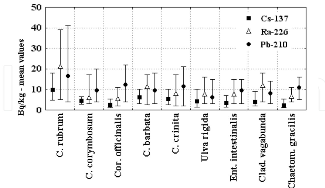
Fig. 10. Comparison of nuclide contents (Bq/kg) in Black Sea algae in different algae species
