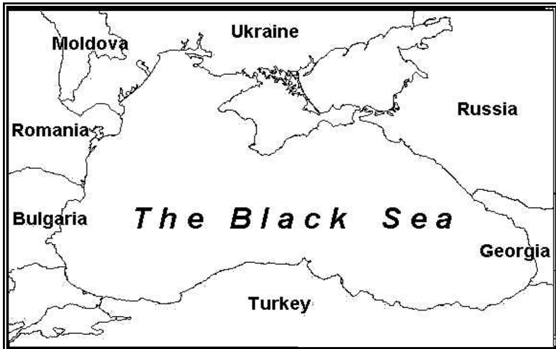
Radionuclide content in Black Sea sediments Gamma Spectroscopy
