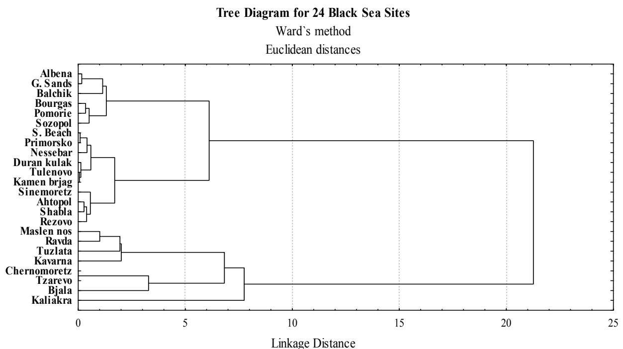
Fig. 7. Tree diagram of Black Sea sediments depending on radionuclide content.
