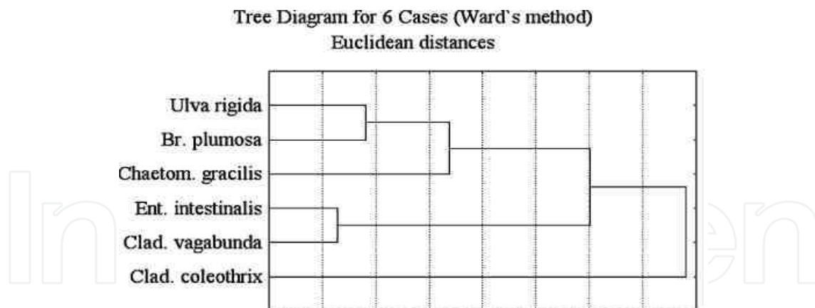
Fig. 15. Tree diagram for heavy metal content in green algae species
