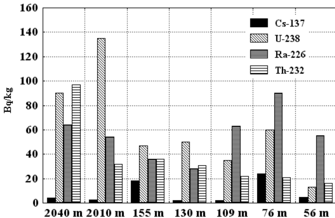
Fig. 6. Mean nuclide content in deep-sea sediment samples
