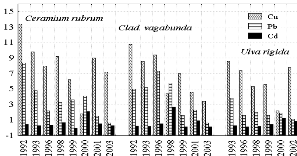
Fig. 13. Seasonal variations of HM concentrations (mg/g) in three alga species
