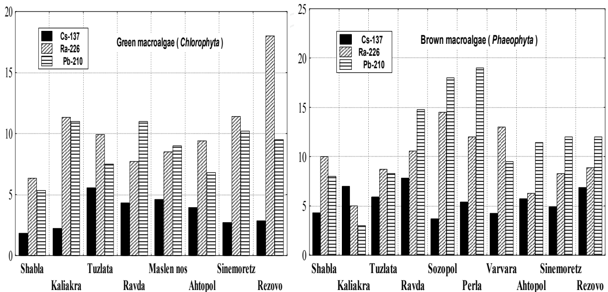
Fig. 8. Nuclide contents (Bq/kg) in green and brown algae
