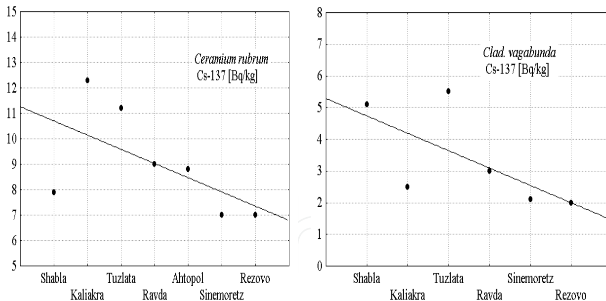
Fig. 11. 137 Cs content in macroalgae – local variations
