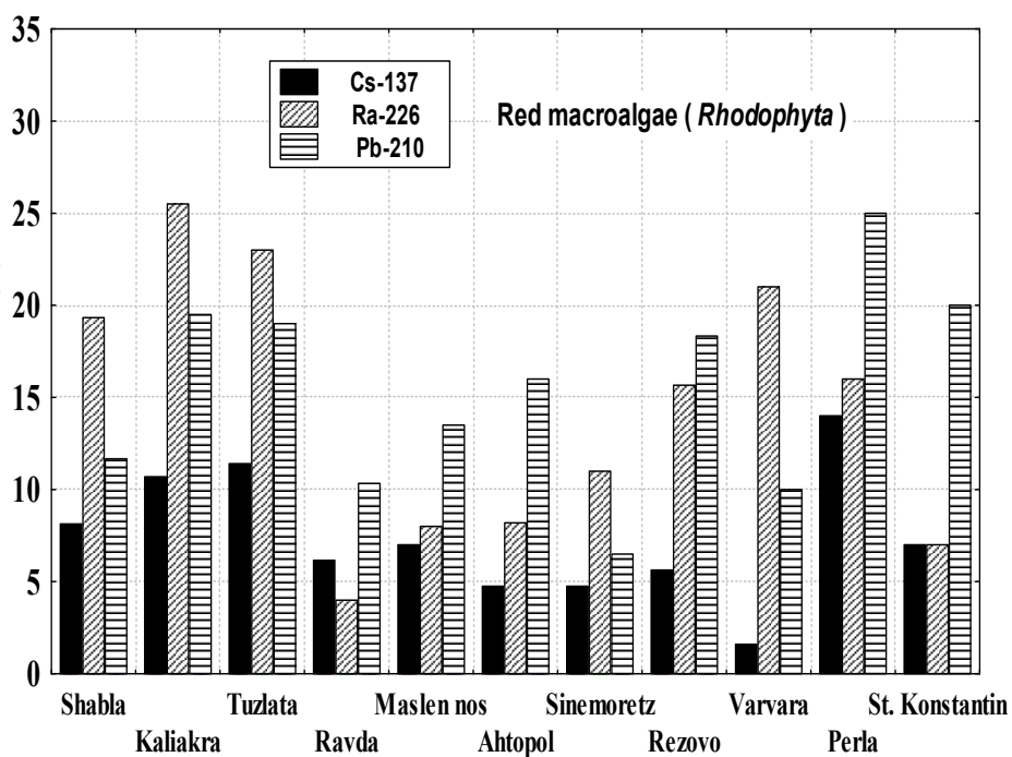
Fig. 9. Nuclide contents (Bq/kg) in Black Sea macrophytes - Rhodophyta
