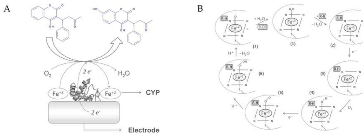
Fig. 17. A) Schematic representation of the CYP2C9 biosensor and the electrochemical oxidation of warfarin catalyzed enzymatically (adapted from Bistolos et al., 2005). B) Catalytic cycle of the CYP heme group and the reactions of the oxidation process (adapted from Lohmann & Karst, 2008).
