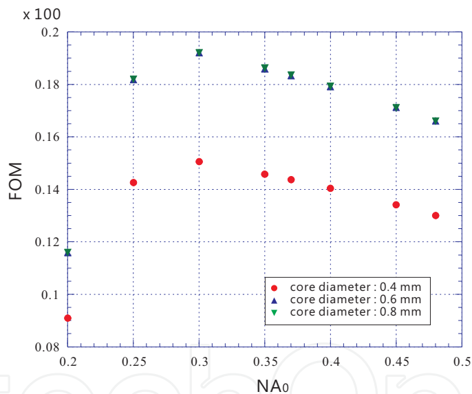
Fig. 6. Calculated values of FOM as a function of NA_0 . The solid circles indicate the values at \phi_0 = 0.4 mm, the solid triangles are the values at \phi_0 = 0.6 mm, and the solid inverse triangles are the values at \phi_0 = 0.8 mm.
