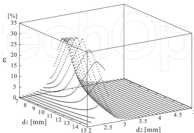
Fig. 7. Calculated values of \epsilon as functions of d_1 and d_2 for given values of NA_0 = 0.37 and \phi_0 = 0.6 [mm].
