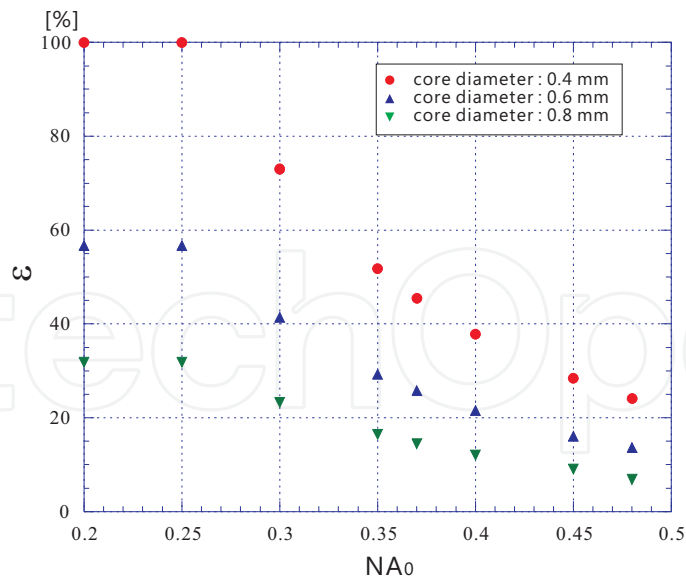
Fig. 5. Calculated values of coupling efficiency \epsilon as a function of NA_0 . The solid circles indicate the values at \phi_0 = 0.4 mm, the solid triangles are the values at \phi_0 = 0.6 mm, and the solid inverse triangles are the values at \phi_0 = 0.8 mm.
