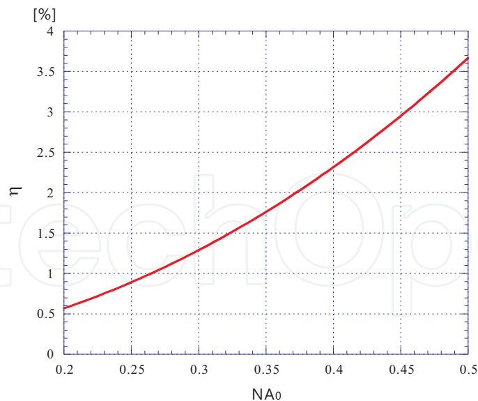
Fig. 3. Calculated values of collection efficiency as a function of NA_0 at n_w=1.33
