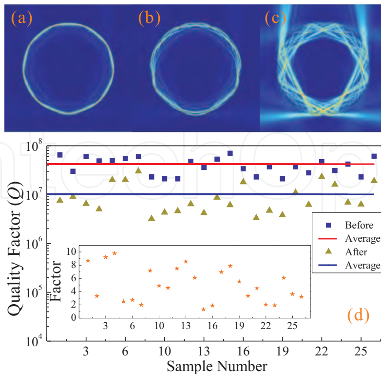
Fig. 10. (a), (b) and (c) The electric intensity distribution of three typical modes in the spot-packaged microsphere. (d) Tested Q of different microspheres before and after the spot-package. Insets: The decreased factor of the Q corresponds to different samples.
