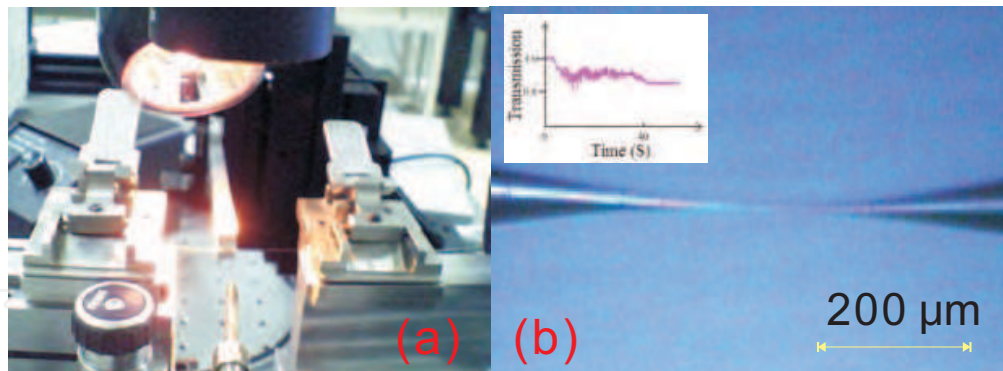
Fig. 2. (a) Tapered fiber fabrication setup in our lab. (b) Typical micrograph of a taper, insets: transmission power monitoring during taper fabrication.
