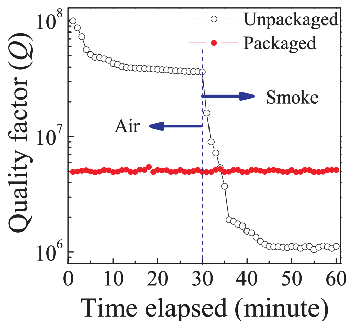
Fig. 7. Tested Q versus elapsed time of a microsphere coupling system in the air and in the smoke, for un-packaged (in black) and packaged (in red) samples, respectively.
