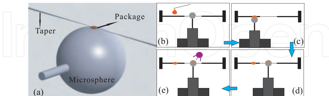
Fig. 8. (a) The schematic diagram of the spot-packaged microsphere-taper coupling system. (b)-(e) Illustration of the spot-package process. Red color represents the package glue.
