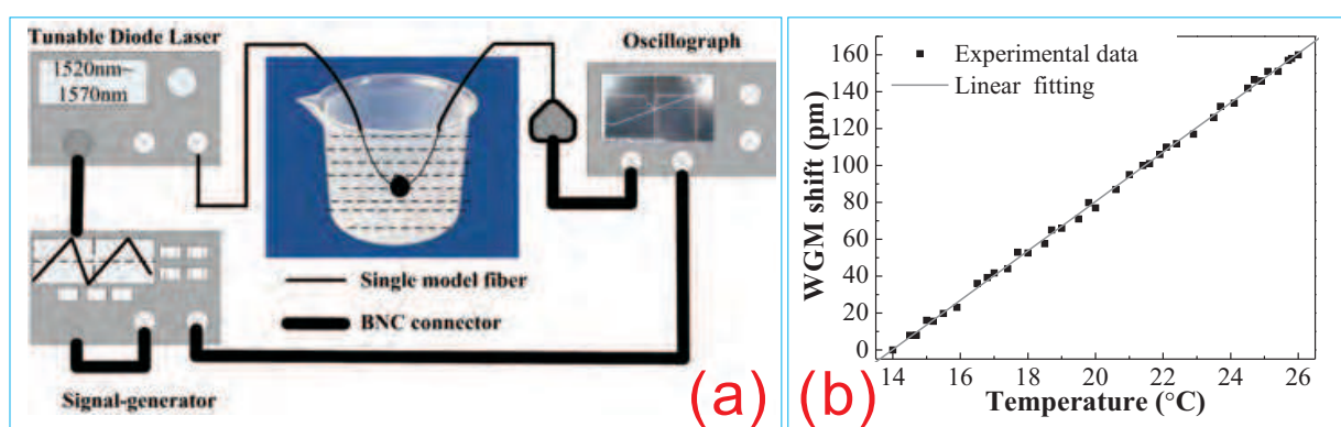
Fig. 11. (a) Temperature testing setup used in our experiments. (b) WGM wavelength shifts as a function of the surrounding temperature, in NaCl resolution and in pure water, respectively.
