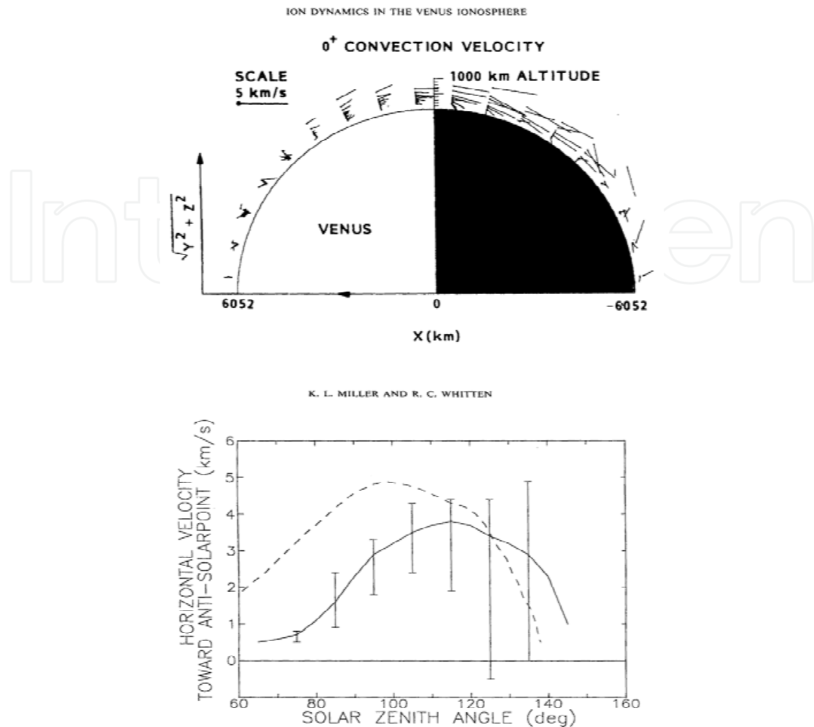
Fig. 5. (upper panel) Average velocity vectors measured in the Venus upper ionosphere with the PVO spacecraft and projected in cylindrical coordinates (the solar wind arrives from the left) 8 . (lower panel). Speed values of the ionospheric particles that move across the terminator at 400 km altitude 9 .
