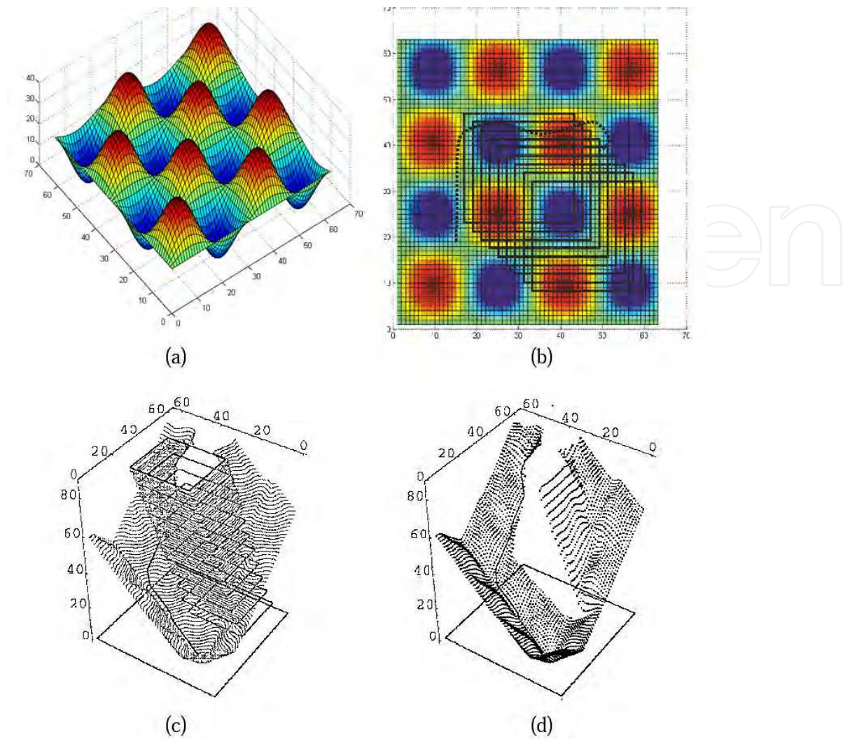
Fig. 7. (a) the terrain definition, (b) a squared object moves across the scene. (c) \alpha(u, t) for different values of t representation (d) Back tracking from the final point toward the starting one along the estimated geodesic path
