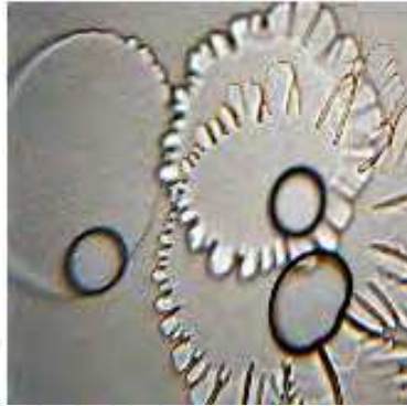
Fig. 1. A typical Tyndall figure (Liquid snowflake)
