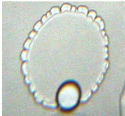
Fig. 2. Liquid snow flakes formation starting from a circle and the evolving, accordingly to linear instabilities with sinusoidal perturbations
