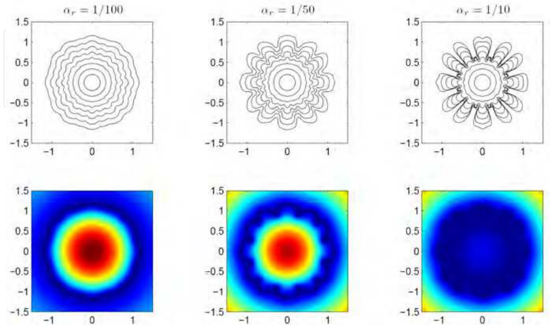
Fig. 3. on the top row: different snapshots of the zero level set evolution varying the relative absorption \alpha_r ; instead on the bottom line different level set values (different temperatures) are presented for the larger curve of the row above
