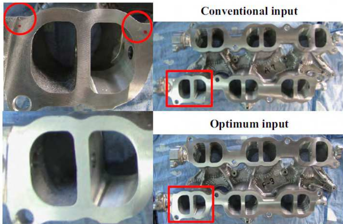
Fig. 14. Experimental results with conventional input and optimum input
