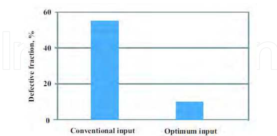
Fig. 15. Defect fraction of machining surface
