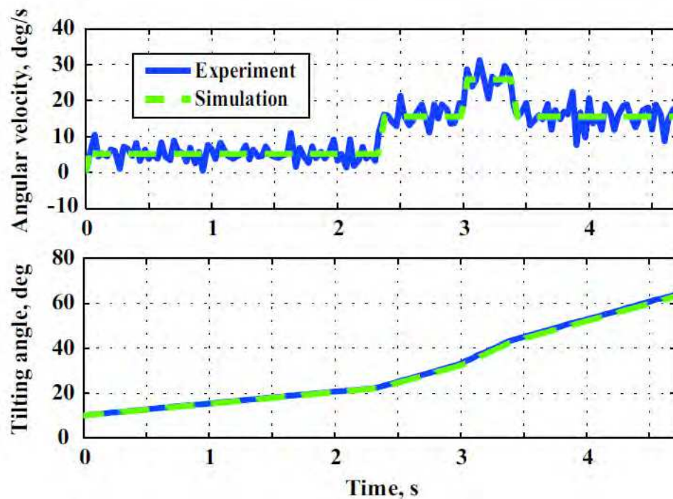
Fig. 4. Result of identification of actual pouring machine.
