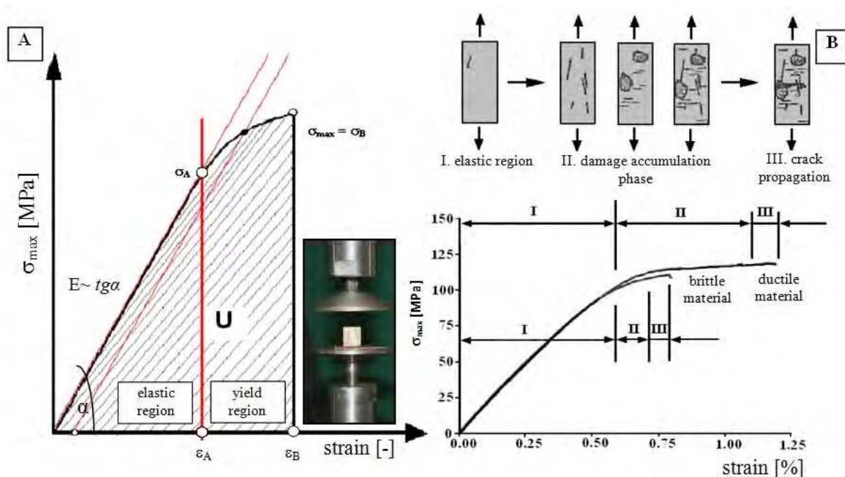
Fig. 3. A. Stress-strain dependency and mechanical parameters such as: Young modulus, ultimate and yield stress and strain energy U, B. changes in integrity of cancellous bone sample during different phase of uniaxial compression test
