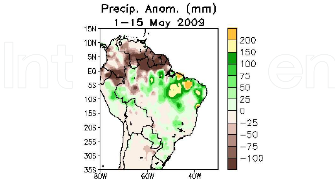
Fig. 15. Precipitation anomalies (mm) for 1-15 May 2009. Anomalies are departures from the 1979-2010 base period.
