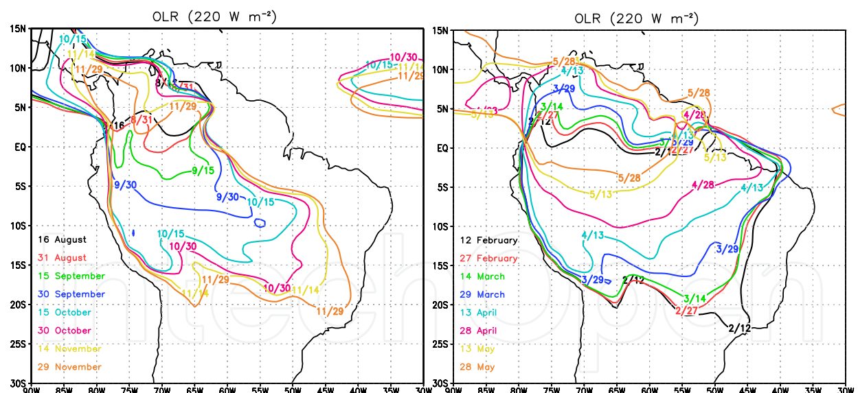
Fig. 10. Time onset and end dates for the wet season in the monsoon core region (Central Brazil) based on OLR less than 220 \text{ W m}^{-2} .
