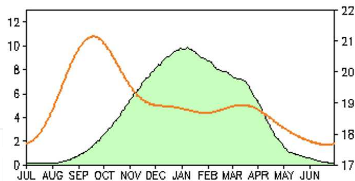
Fig. 9. Mean (1979-1995) daily precipitation (mm) for central Brazil ( 12.5^{\circ} - 17.5^{\circ} S, 47.5^{\circ} - 52.5^{\circ} W) (shaded in green), and 850-hPa temperature (degrees C, red curve). The 850-hPa temperature data are taken from the R1 data archive.
