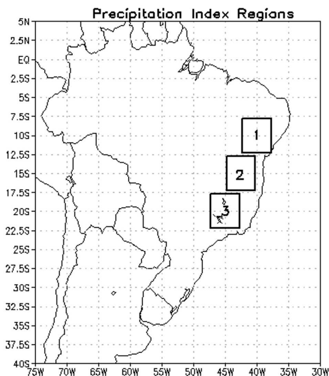
Fig. 19. Precipitation Index for selected regions.
