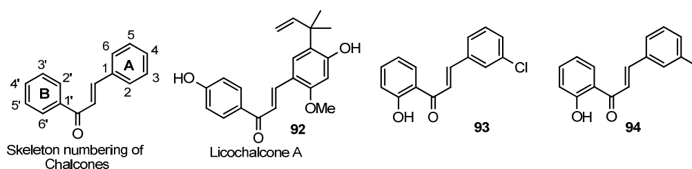
Fig. 8. Chalcones with anti-TB activities
