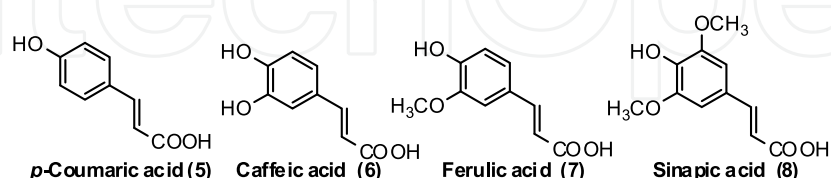
Fig. 2. Cinnamic acid and its natural phenolic-analogues
