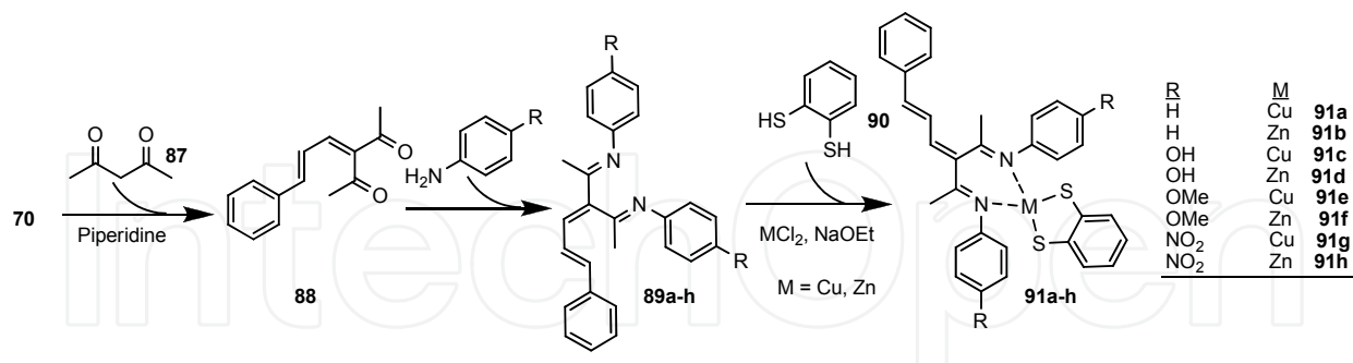
Scheme 15. Preparation of Cu(II) and Zn(II) complexes starting from cinnamaldehyde
