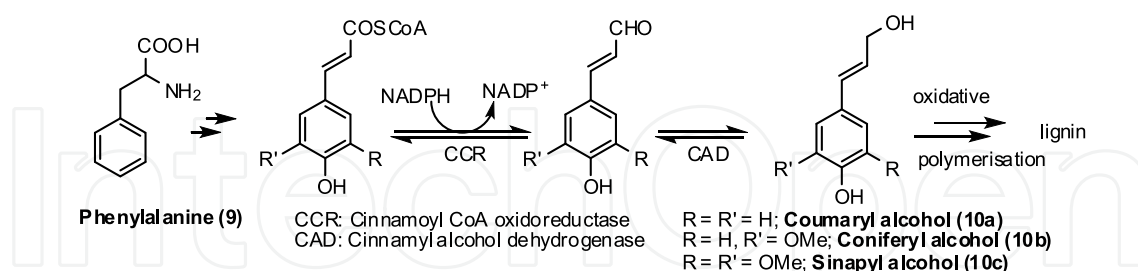
Scheme 1. Lignin biosynthesis pathway
