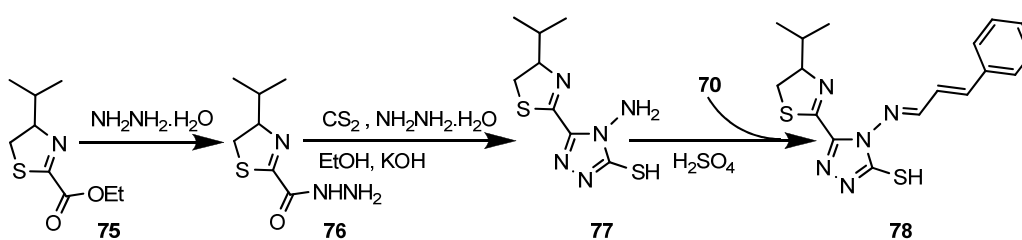
Scheme 12. Synthesis of 2-substituted-5-[isopropylthiazole] clubbed 1,2,4-triazole
