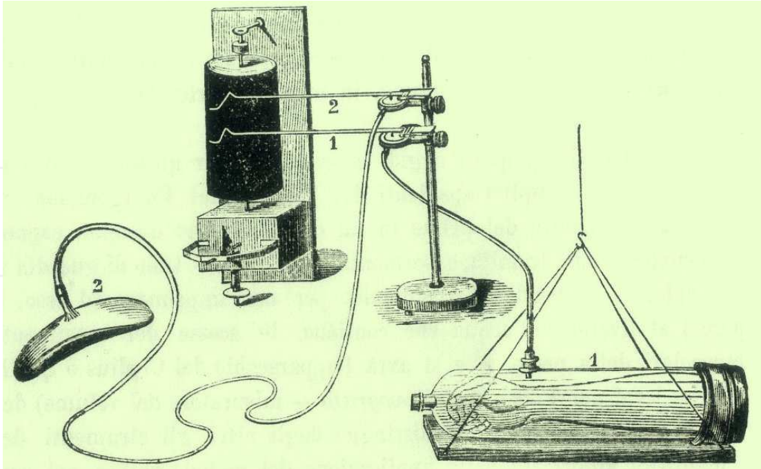
Fig. 3. Mosso's devices for recording the blood volumes in arm and brain. Source: Patrizi (1896).
