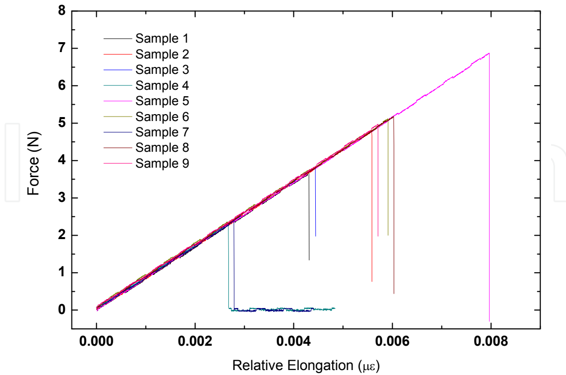
Fig. 3. Force versus strain experimental data for each sample of standard optical fiber without the acrylate protective coating.
