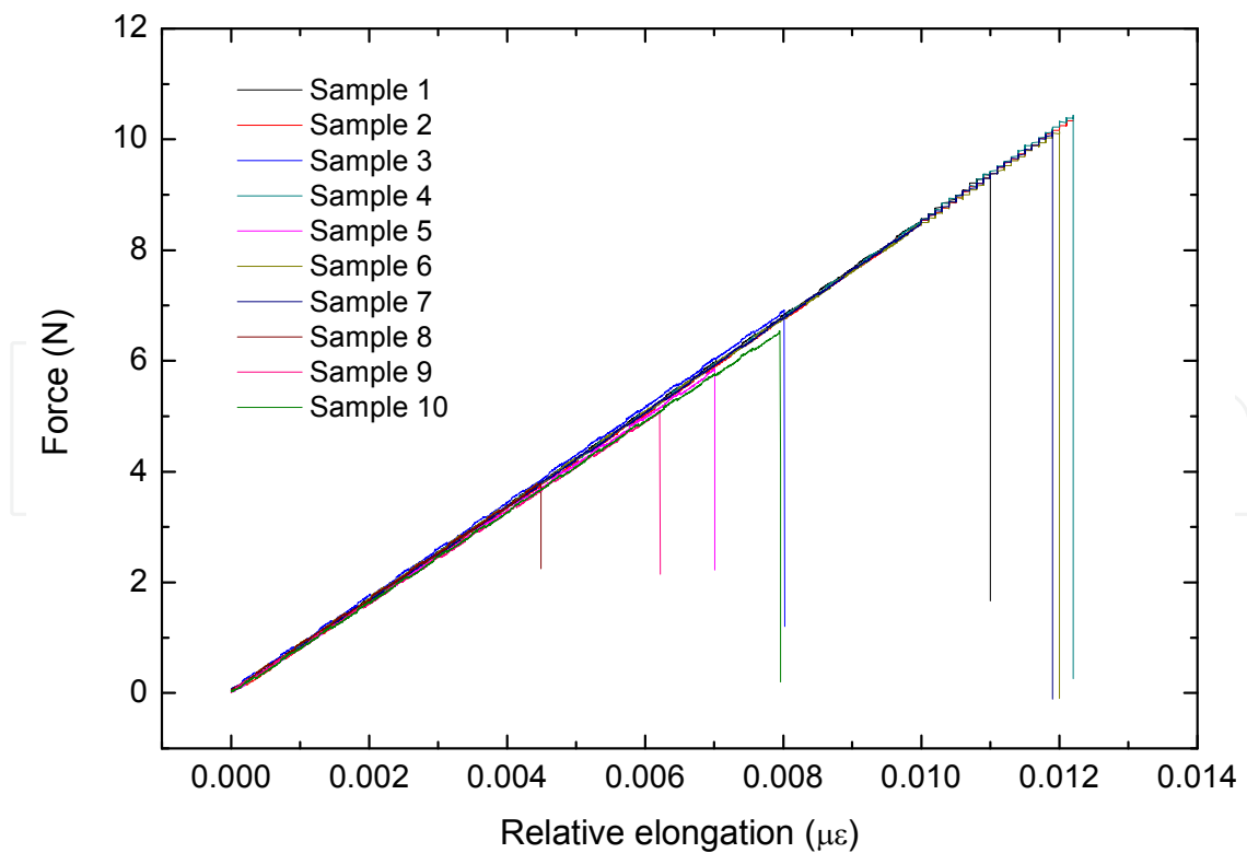
Fig. 4. Force versus strain experimental curve for the ten samples of photosensitive optical fiber without the acrylate protective coating.
