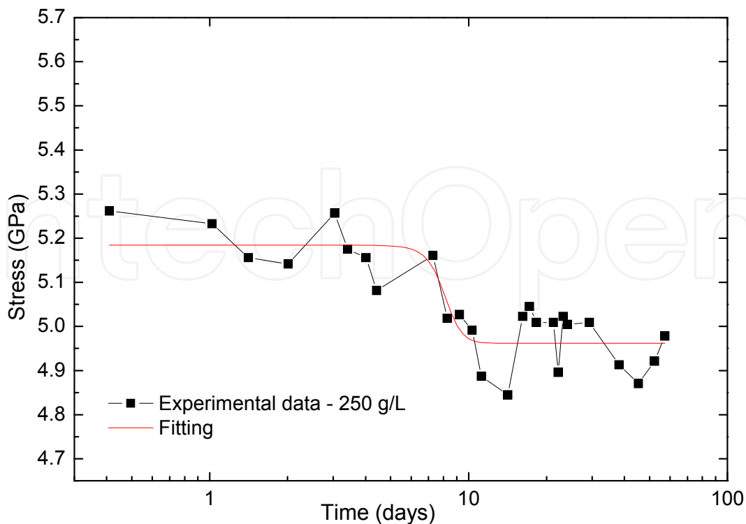
Fig. 7. Fracture stress along time for the fibers aged in the a) 35, b) 100 and c) 250 g/L NaCl solutions and fitting to the Boltzmann function.
