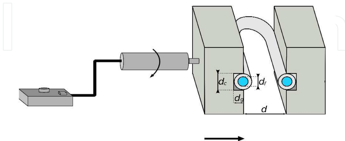
Fig. 5. Illustration of the experimental setup used to measure the fiber fracture stress.
