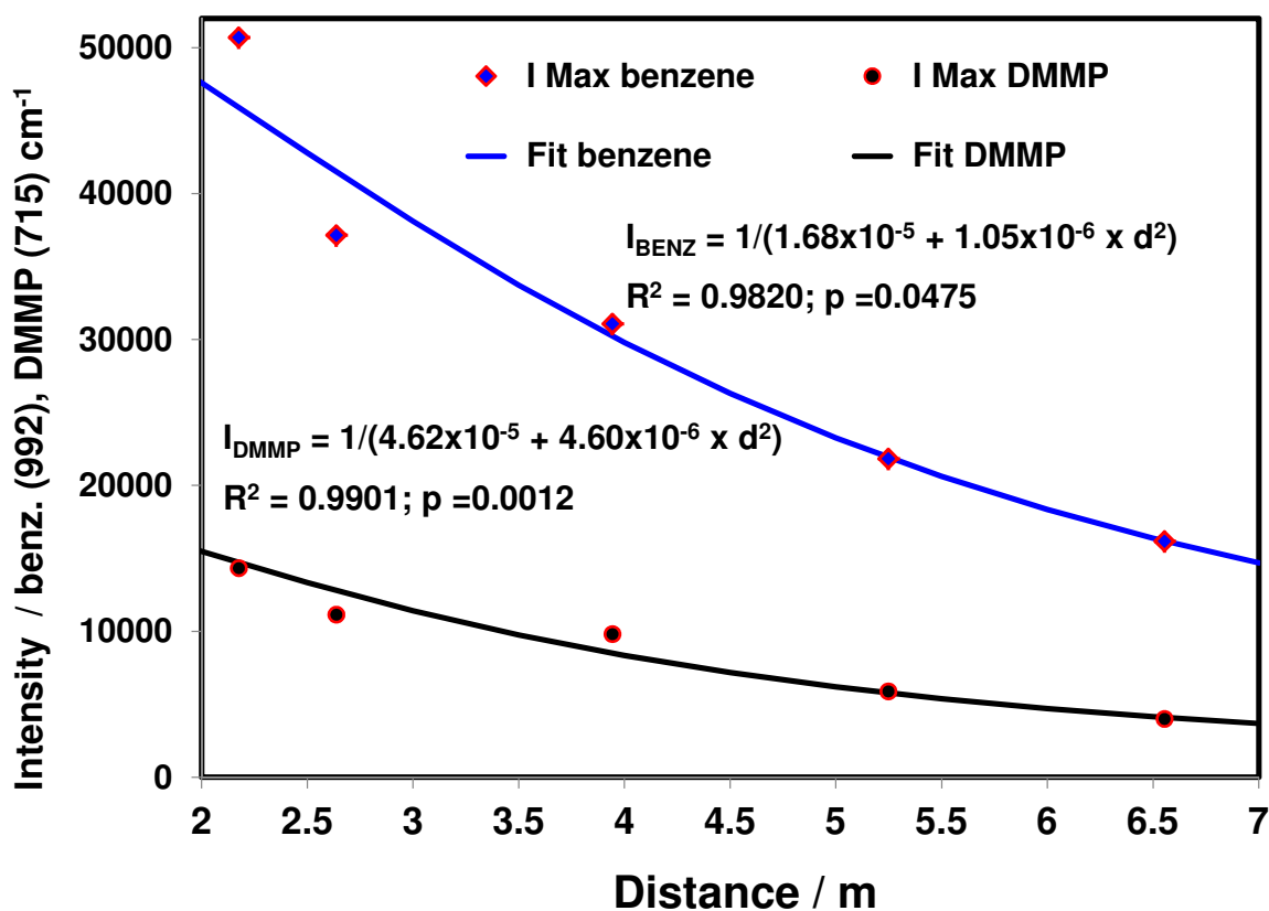
Fig. 20. Dependence of Raman Shift signal (vibrational band intensities) with standoff distance for benzene and DMMP using the 363.8\text{ nm} excitation line from a UV-argon ion laser.
