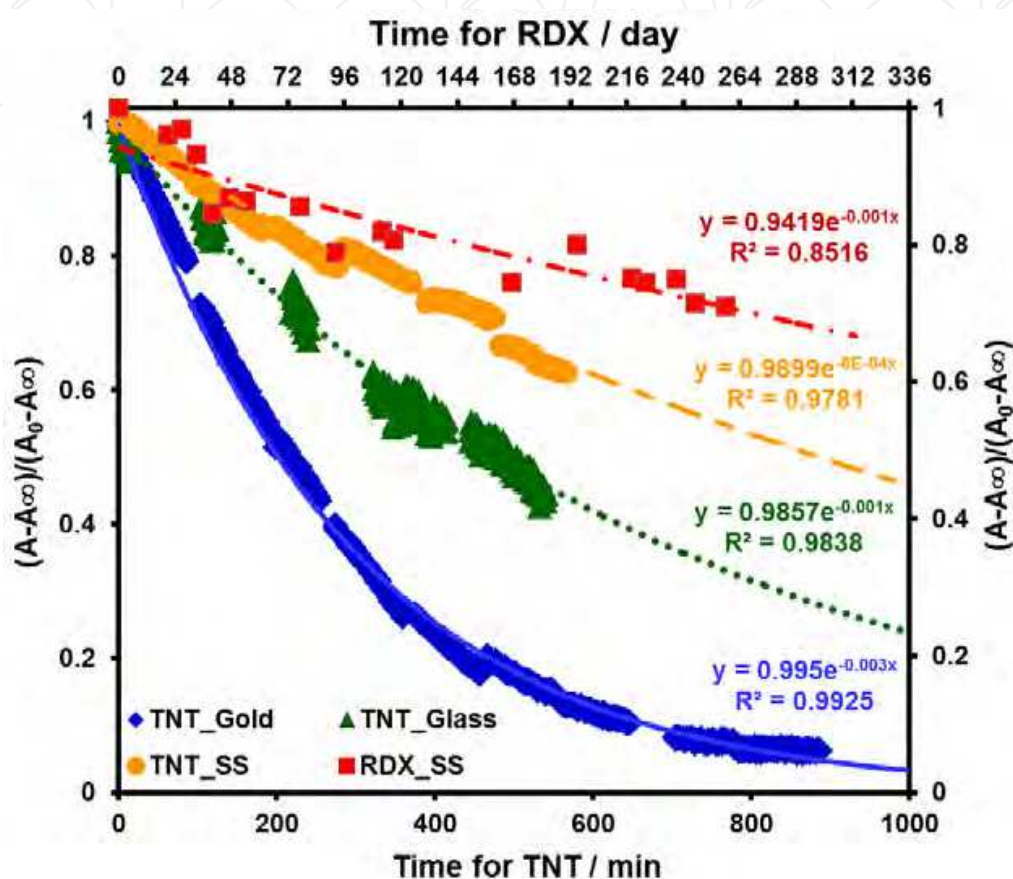
Fig. 8. Plots of (A - A_{\infty}) / (A_0 - A_{\infty}) vs. time for surface sublimation for: TNT on gold-silicon ( \blacklozenge ); TNT on glass ( \blacktriangle ), TNT on stainless steel ( \bullet ) and RDX on stainless steel ( \blacksquare ).
