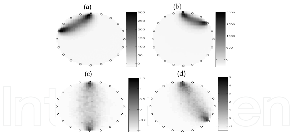
Fig. 10. (“banana shaped”) photon distributions through the homogeneous 3D head model between the single source and various detectors 4, 17,10, and 13 from (a) to (d) respectively.
