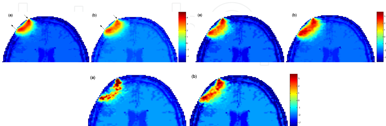
Fig. 11. Spatial sensitivity profiles of photons in the realistic 3D head model. Depth sensitivity is limited by the presence of endogenous chromophores such as haemoglobin, water and cytochrome. The optical path travelled by photons between the source and the detector is strongly dependent to the thickness and the optical properties of the superficial tissues and the 'void' region, which is the CSF of the head. Data measurements from multiple source-detector separations provide overlapping measurement from a limited area. These are used for tomographic image reconstruction utilising 3D models (Mansouri et al., 2010).
