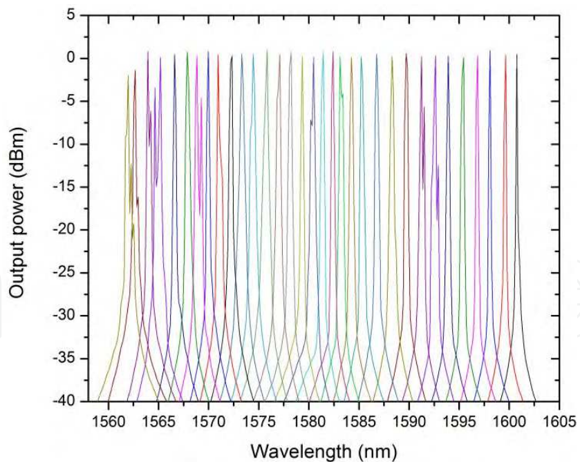
Fig. 20. Tuning range of 39nm, output power versus wavelength.
