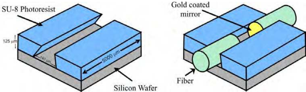
Fig. 7. Wavelength tuning SU-8 device.
