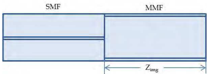
Fig. 1. A schematic diagram in which the multimode interference effect takes place in optical fibers.
