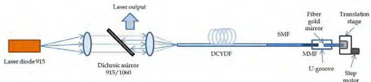
Fig. 6. Schematic diagram of the experimental setup.
