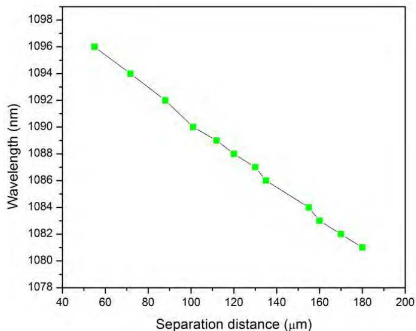
Fig. 8. Experimental results of displacement of facet mirror fiber versus emitted laser wavelength.
