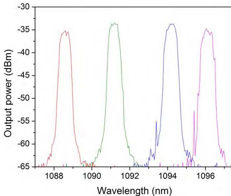
Fig. 5. Total optical tuning range of a DCYFL.
