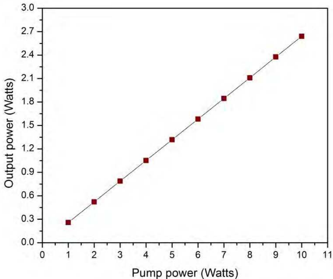
Fig. 23. Erbium results, output power versus pump power.
