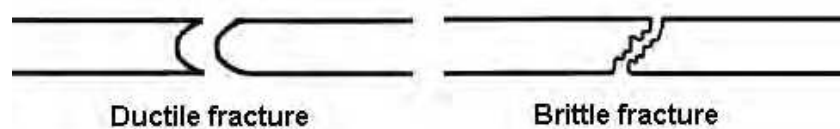
Fig. 7. Typical fractures of a ductile material and a brittle material.
