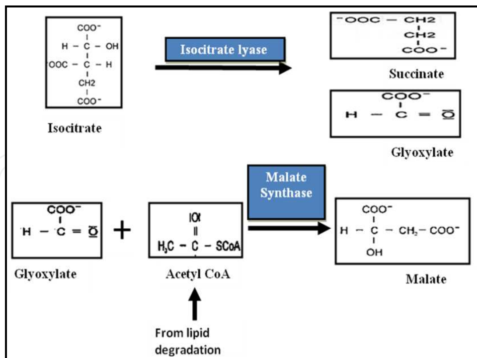
Fig. 2. Reaction scheme of glyoxylate shunt.
