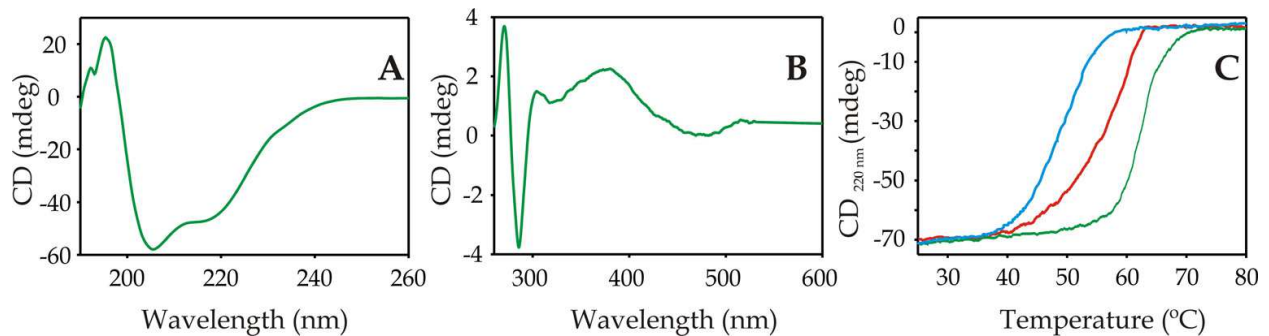
Fig. 5. Structural study of FNRs by CD spectroscopy. A and B) Typical CD spectrum in the far-UV (A) and near-UV (B) regions of plant FNR properly folded (pea FNR). C) Thermal unfolding of different FNRs. From these curves it is possible to estimate the parameters associated to FNR stability. Green: pea FNR; red: E. coli FNR; blue: Xanthomonas axonopodis FNR.
