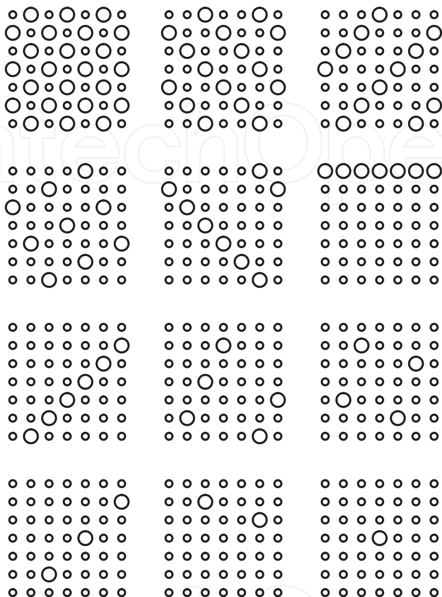
Fig. 7. Networks with different stoichiometries, from left to right, top to bottom, s = \{1.04, 2.06, 3.08, 4.44, 5.125, 6, 7.16, 8.8, 11.25, 15.33, 23.5, 48\} , and equal number of harvesting complexes.
