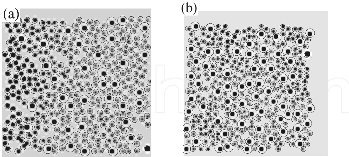
Fig. 12. Contour plots for dissipation in LLI (a) and HLI (b) membranes. Greater contrast means higher values for dissipation. The simulation is shown after 10^6 excitations were absorbed by the membrane with rate \gamma_A .
