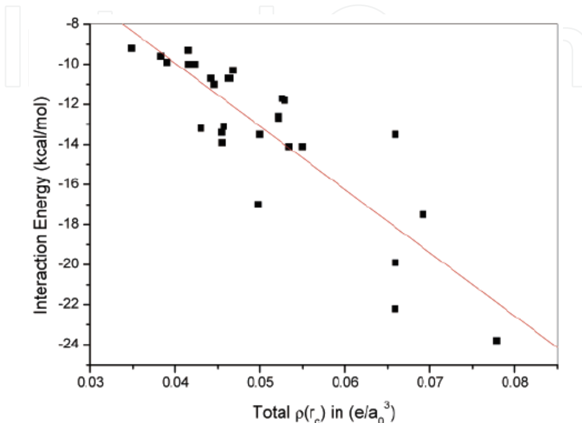
Fig. 10. Relationship between the interaction energy and total \rho(r_c) of the DNA base pairs.
