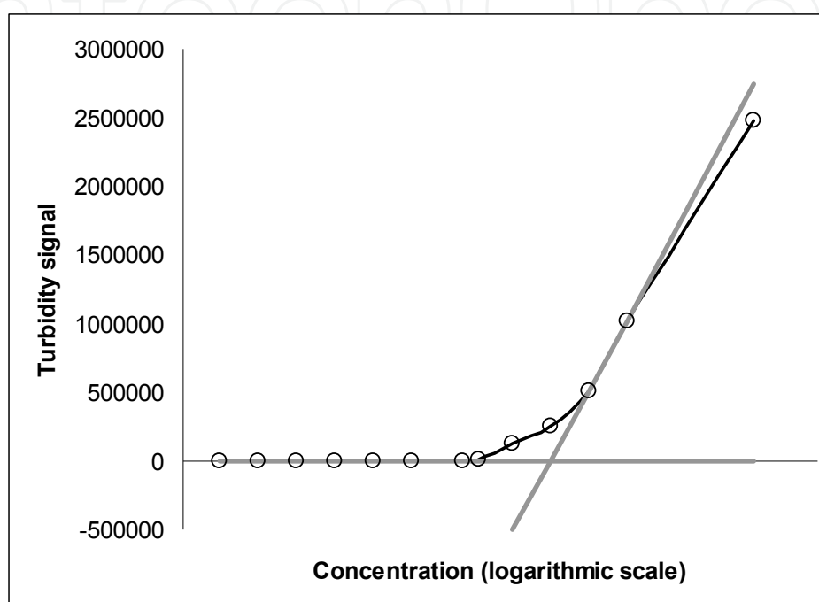
Fig. 3. The method for finding kinetic solubility.
