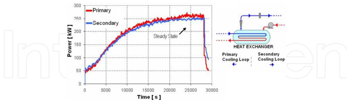
Fig. 21. Thermal power evolution in the cooling system (Zacarias Mesquita and Cesar Rezende, 2007).
