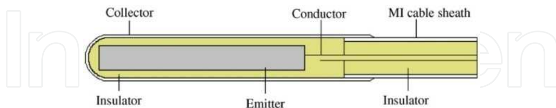
Fig. 9. Schematic diagram of self powered neutron detector
