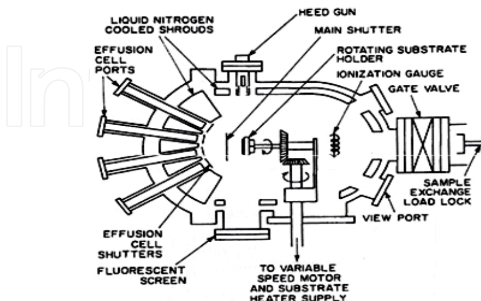
Fig. 3. Cut-away view of a modern MBE system viewed from the top (Chang & Kai, 1994).
