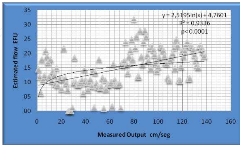
Fig. 12. Polinomial regression plot
