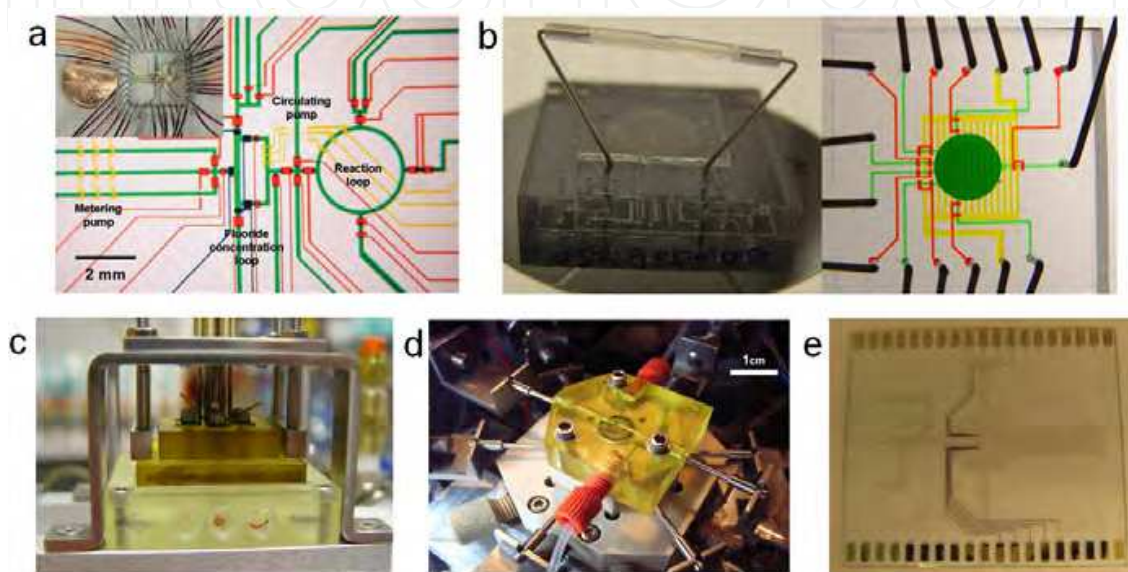
Fig. 4. Batch-format microfluidic platforms for synthesis of PET tracers. (a) Silicone rubber chip (Lee et al. 2005). (b) Scaled-up silicone rubber chip (Elizarov et al. 2010). (c) Chemically-inert pDCPD chip (van Dam et al. 2007) mounted in reagent loading interface and illustrating microvalve actuators. (d) “Open” chip (Bejot et al. 2010) mounted on reagent loading interface and illustrating mechanical actuators for integrated valves. (e) All-electronic EWOD microfluidic chip (Keng et al. 2011).
