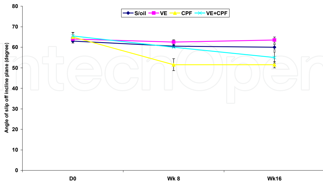
Fig. 4. Effect of chronic administration of soya oil, vitamin E and/or chlorpyrifos on the dynamics of incline plane performance in Wistar rats.
