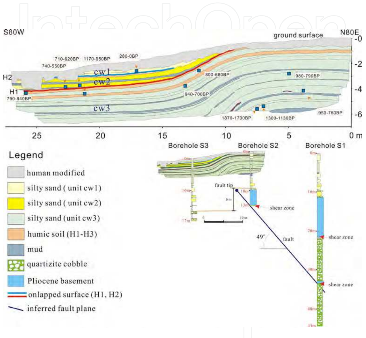
Fig. 2. The contact of alluvial deposits and humic soil (H1 and H2) occurs a distinct onlapped structure interpreted to represent a paleoearthquake event. Radiocarbon dates are used to constrain the timing of S1 and S2 paleoseismic events. Fault dip of fault depends on correlation between the borehole S1 and S2 of 49° dips. The Pliocene formation shows inclined bedding plane and is weakly sheared. The fluvial cobble deposits between boreholes S2 and S3 offset about 6-m high in both sides of the fold scarp.
