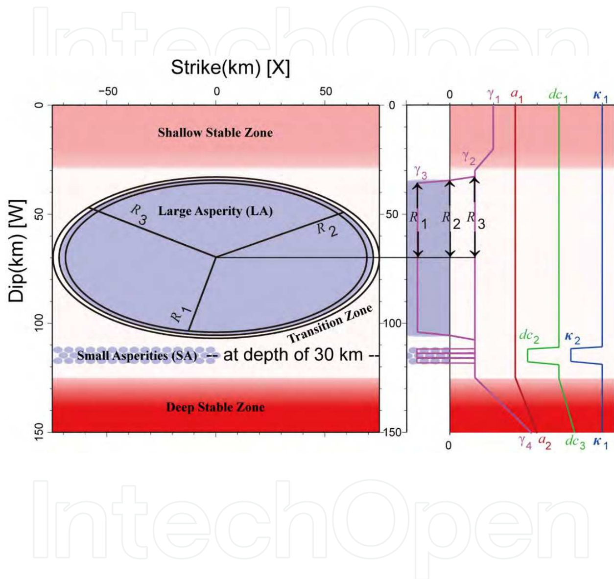
Fig. 3. Frictional parameters ( a , \gamma (= a-b) , d_c , \kappa ) (See Eq. (2)) as functions of distance along the dip direction from the surface on the plate boundary, where (a_1, a_2) = (2, 5) [\times 10^{-3}] , (\gamma_1, \gamma_2, \gamma_3, \gamma_4) = (0.5, 0.01, -0.3, 4.9) [\times 10^{-3}] , (d_{c1}, d_{c2}, d_{c3}) = (10, 0.43, 100) [\text{mm}] , and (\kappa_1, \kappa_2) = (1.0, 0.1) . Half the length of the minor axis (along dip) of the elliptical asperity takes the following values: for LA, (R_1, R_2, R_3) = (35, 36.25, 37.5) [\text{km}] and for SA, (r_1, r_2, r_3) = (1.33, 1.5, 1.67) [\text{km}] , where the aspect ratios for LA and SA are 2.0 and 1.5, respectively. The distance between central points of SA along strike and dip direction is 2 and 2.5 km, respectively. This figure is developed from Ariyoshi et al. (2011a).
