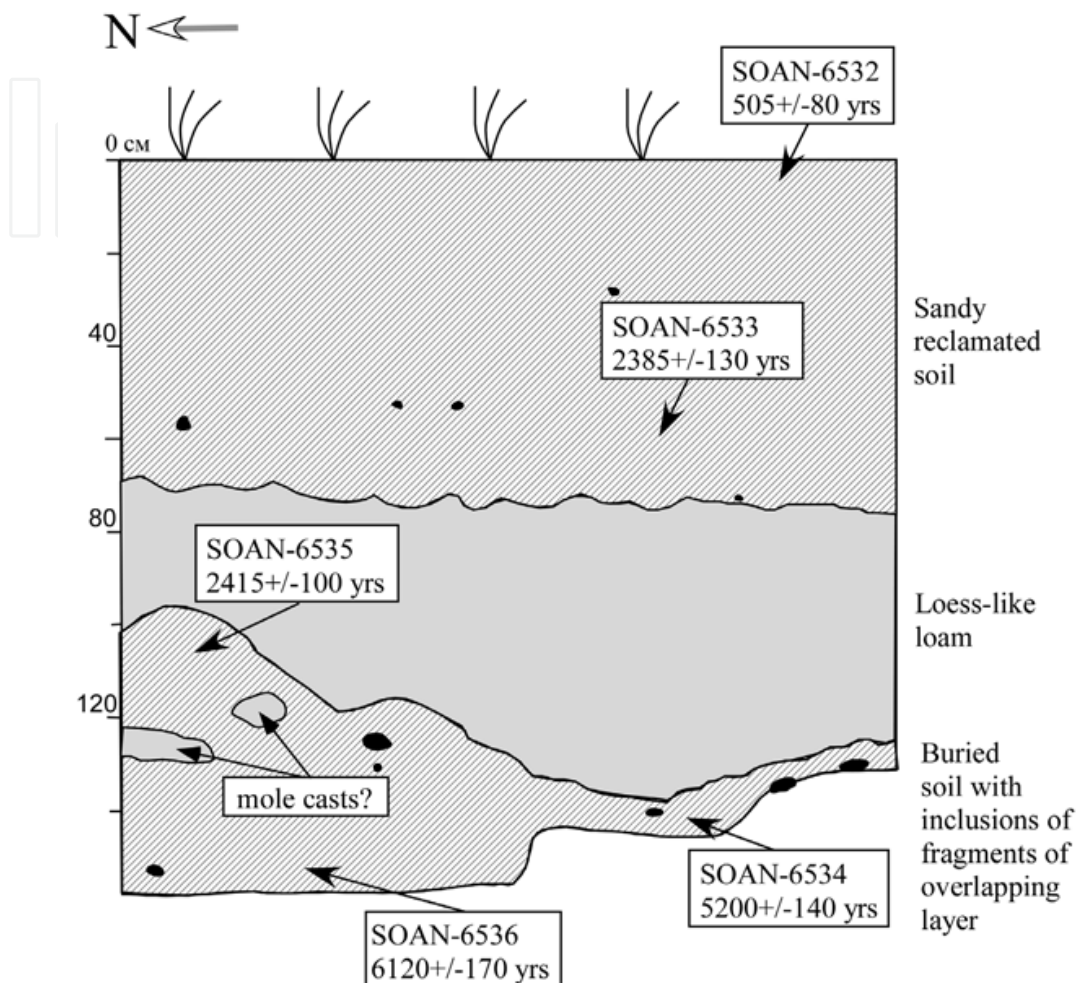
Fig. 20. Bore pit 3 at the Sary-Bulak test site. Recent reclaimed soil is separated from the buried soil by the «colluvial wedge». Black stains in the drawing are pebbles of average roundedness.
