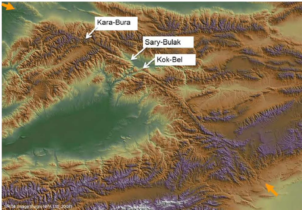
Fig. 2. Digital map of relief of the western Tian Shan. The locations of the investigated test sites are shown in the map.
