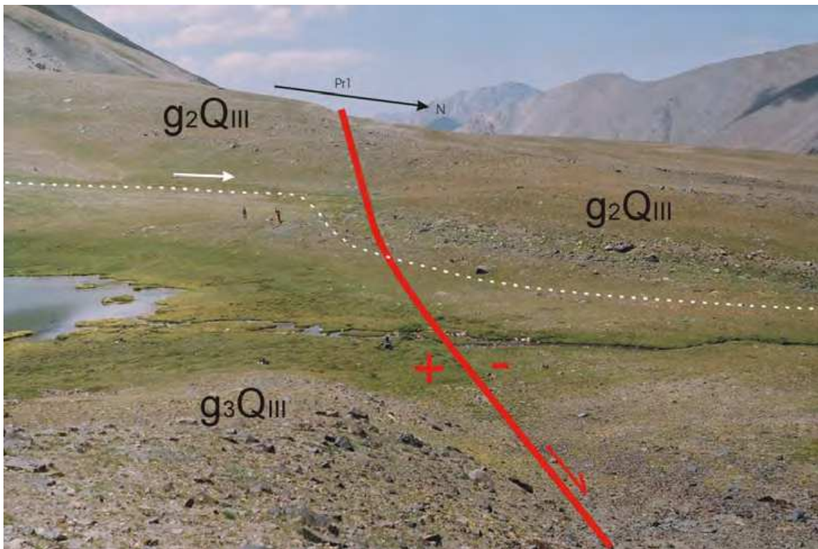
Fig. 10. Photo of the Kara-Bura polygon. View north-westward. The red line is the TFE, the white dashed line is the dry channel, the arrow Pr1 is the profile line in Fig. 9, g_{2Q_{III}} is a recessional moraine of the middle of Late Pleistocene. g_{3Q_{III}} is a recessional moraine of the end of Late Pleistocene.
