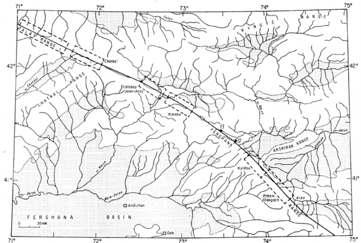
Fig. 1. The map of the Talas-Fergana Fault's line and adjacent territories (modified after Burtman et al., 1996). Dashed rectangulars shows studied portions of the fault. Sedimentary basins are indicated by regular dotty filling. Irregular dotty area shows lakes and reservoirs. Numbers along the fault's line are observation points N12 and 13 from Burtman et al. (1996).
