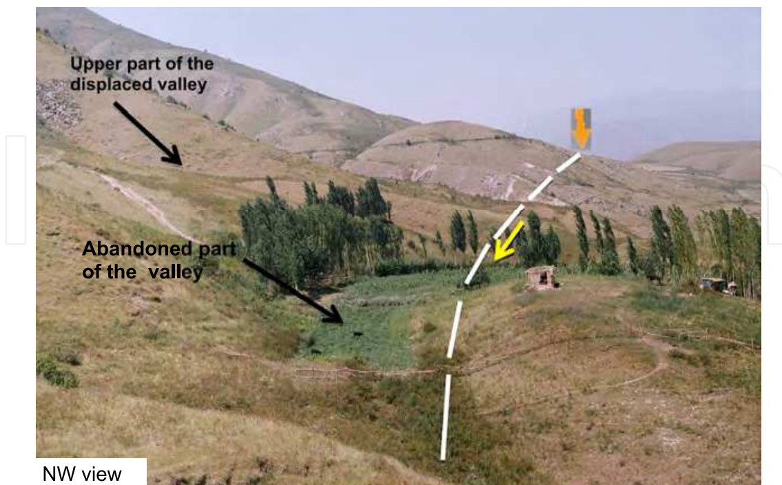
Fig. 18. A fragment of the upper part of the valley of the Sary-Bulak River.
