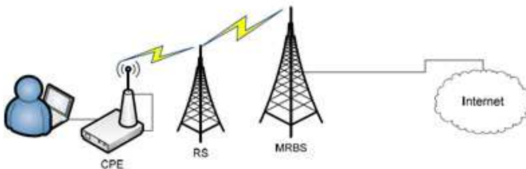
Fig. 16. Two hops topology.
