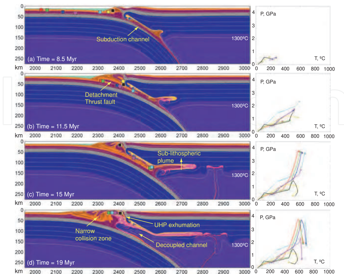
Fig. 5. Enlarged domain evolution ( 1075 \times 275 \text{ km} ) of the model with higher convergence velocity V_x = 10 \text{ cm/y} . Colors of rock types are as in Figure 1. Time (Myr) of shortening is given in the figures. White numbered lines are isotherms in ^{\circ}\text{C} . Small colored squares indicate positions of representative markers (rock units) for which P - T paths are shown (right). Colors of these squares are used for discrimination of marker points plotted in P - T diagrams and do not correspond to the colors of rock types.
