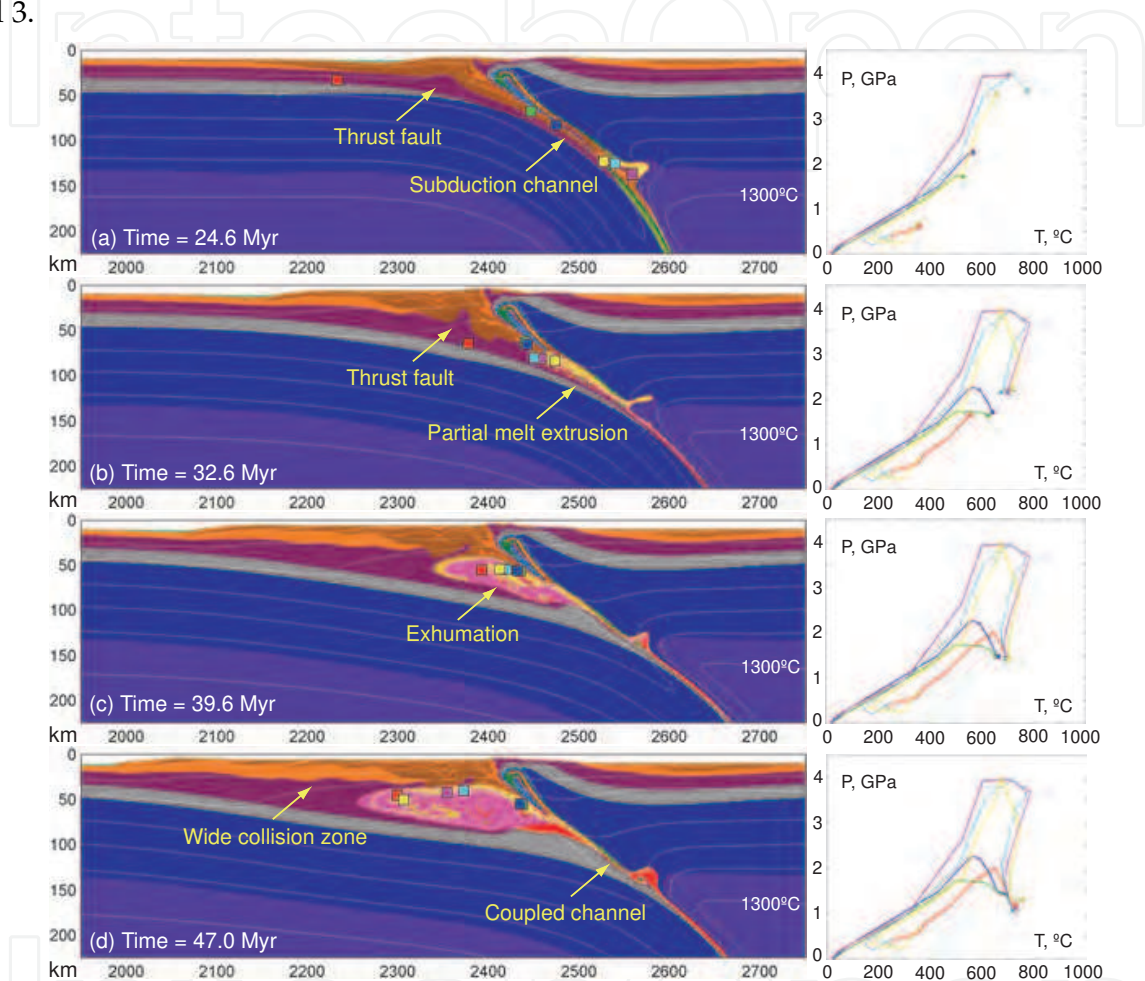
Fig. 4. Enlarged domain evolution (800 × 225 km ) of the model with lower convergence velocity V_x = 2.5 \text{ cm/y} . Colors of rock types are as in Figure 1. Time ( Myr ) of shortening is given in the figures. White numbered lines are isotherms in °C. Small colored squares indicate positions of representative markers (rock units) for which P-T paths are shown (right). Colors of these squares are used for discrimination of marker points plotted in P-T diagrams and do not correspond to the colors of rock types.
