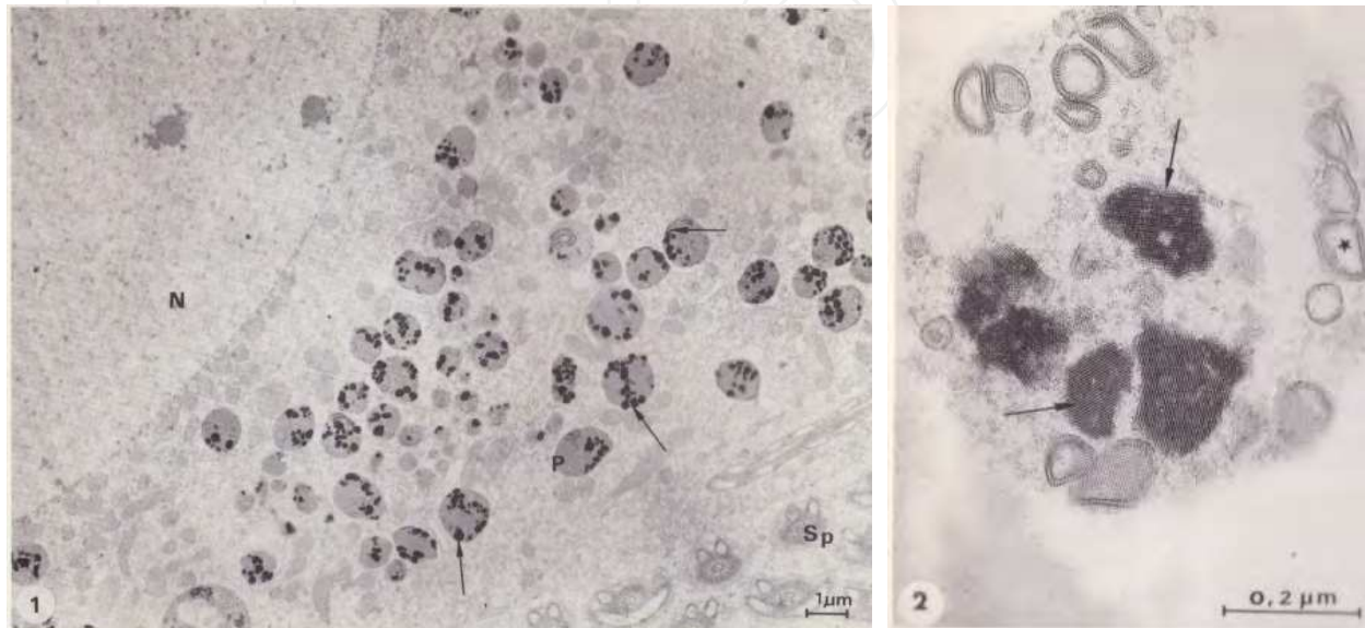
Fig. 1. (1) Ultrastructure of the ovotestis of Planorbarius , at the last stage of vitellogenesis. The platelets (P) of the oocyte contain electron-dense of ferritin (arrows), N, nucleus, Sp, cross section of the sperm tails. Unstained osmicated ultrathin sections. X 7800. (2) Detail of a snail platelet. Natural occurrence of crystalline form of ferritin (arrows). Unstained non-osmicated section. X 50 000 (after Quintana et al., 1987).
