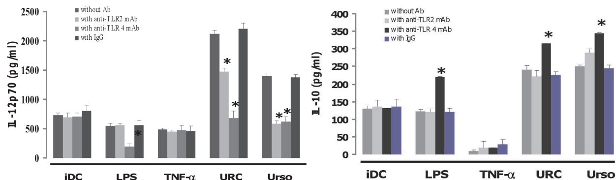
Fig. 3. The production of IL-12p70 by URC-primed dendritic cells and Ursolic acid-primed dendritic cells was inhibited by anti-TLR2 mAb and anti-TLR4 mAb. Dendritic cells were generated by stimulating immature dendritic cells with URC (0.1 \mu M), Ursolic acid (1 \mu M), LPS (100 ng/ml) or TNF- \alpha (25 ng/ml). Cells ( 4 \times 10^4 cells/well) were stimulated with the CD40 L-transfected J558 cells ( 5 \times 10^4 cell/well) for 24 h., the production of IL-12p70 (A), and IL-10 (B) was measured by ELISA in culture supernatants. iDC: immature dendritic cells. Data are the mean \pm S.E.M. of five independent experiments. * P < 0.05 compared without mAb.
