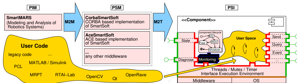
Fig. 13. Two step transformation workflow: Framework Builder view.
