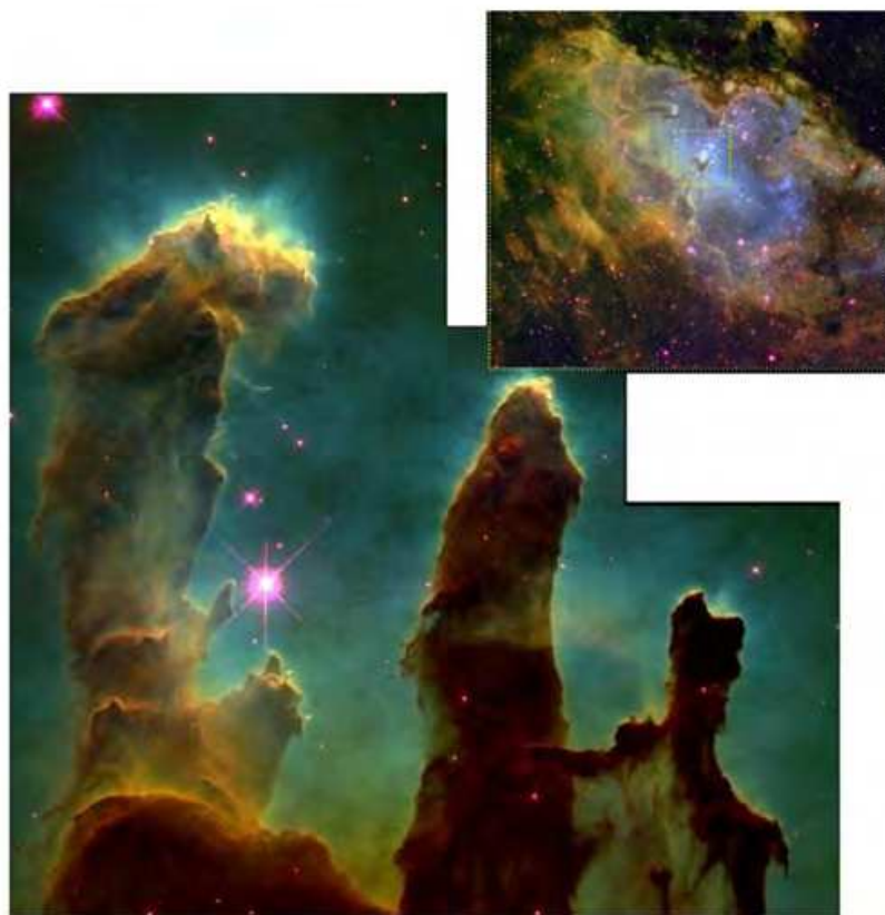
Fig. 1. Photodissociation region known as Gaseous Pillars associated with recent star forming region inside M16 nebulea (Figure inset). The fingerlike structures are the remnants of the molecular clouds which were sculpted by radiation pressure of young stars. (From Hubble Space Telescope 2003)
