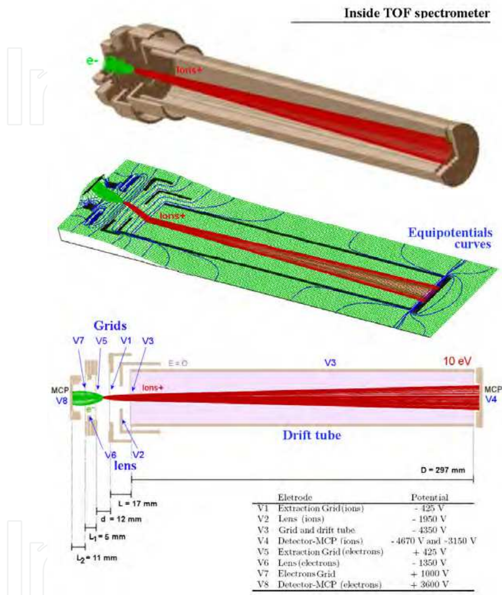
Fig. 3. Particle tracks inside the TOF spectrometers and the potentials employed in the experiments. The simulations were performed using the particle track software SIMION ® .
