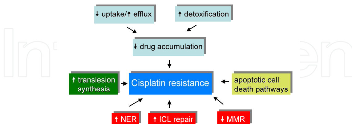
Fig. 2. Mechanisms of resistance towards cisplatin include: Reduced drug accumulation due to changes in drug uptake, efflux or detoxification. Alterations in DNA repair such as increased removal of the damage by nucleotide excision repair (NER) or interstrand crosslink repair (ICL repair) as well as decreased mismatch repair (MMR). Enhanced translesion synthesis (TLS) to tolerate unrepaired cisplatin lesions. Alterations in apoptosis pathways: changes in expression levels of pro- and anti-apoptotic proteins.
