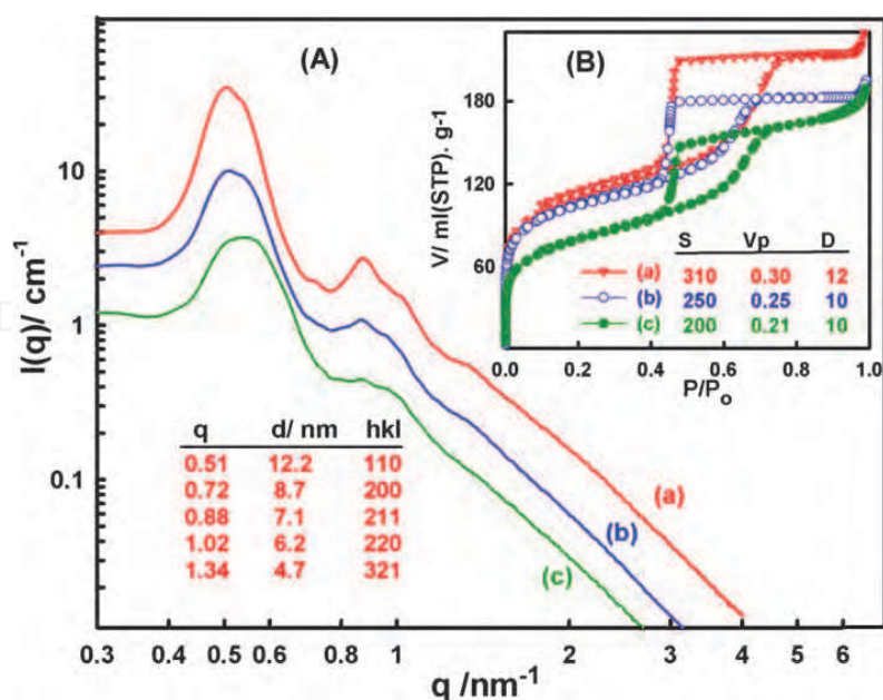
Fig. 11. SAXS (A) and N_2 isotherms (B) of mesofilter membranes based on mesoporous cubic Im3m cage silica NT hybrid AAM before (a) and after (b) modification with TMS groups and after removal of the blocked proteins from the AAM surfaces and pores during the second use of the mesofilters (c) (reprinted from El-Safty, 2011).
