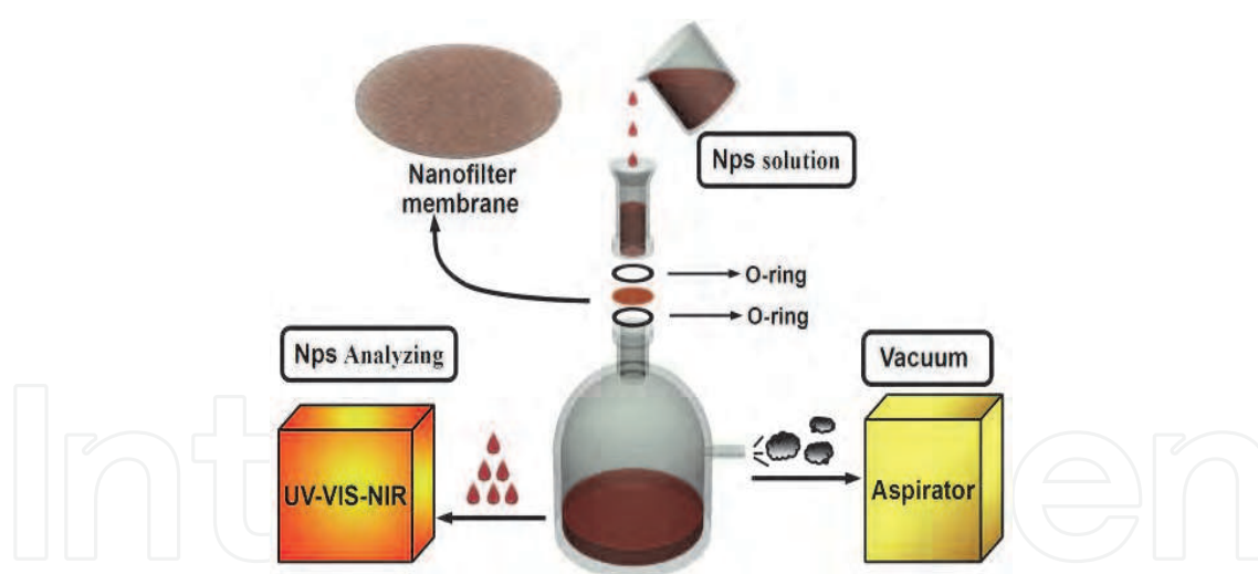
Fig. 10. Schematic diagram of a nanofiltration system used for the synthesis of highly ordered silica NT membrane and the NP filtration (El-Safty et al., 2010, 2011)
