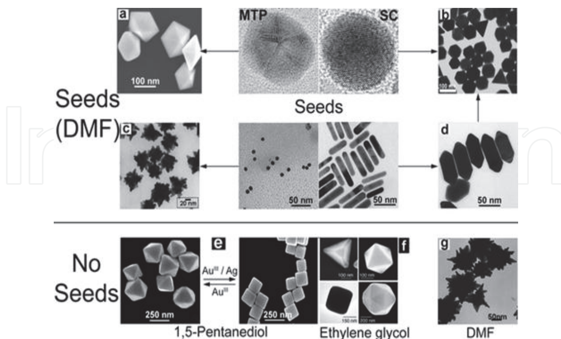
Fig. 1. TEM images of Au NPs with different shapes and sizes synthesized by different pathways (reprinted from Grzelczak et al., 2008).
