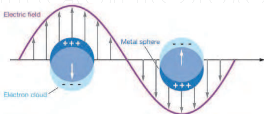
Fig. 5. Schematic diagram illustrating a localized surface plasmon (reprinted from Willets & Duynes, 2007)
