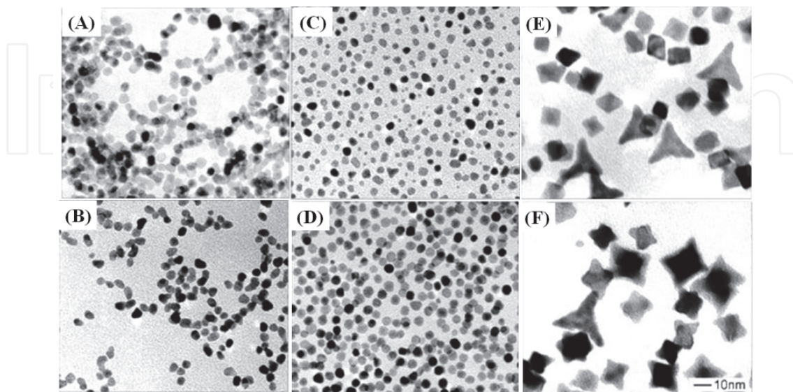
Fig. 2. TEM images of Pt NPs of different shapes and sizes (reprinted from Herricks et al., 2004)
