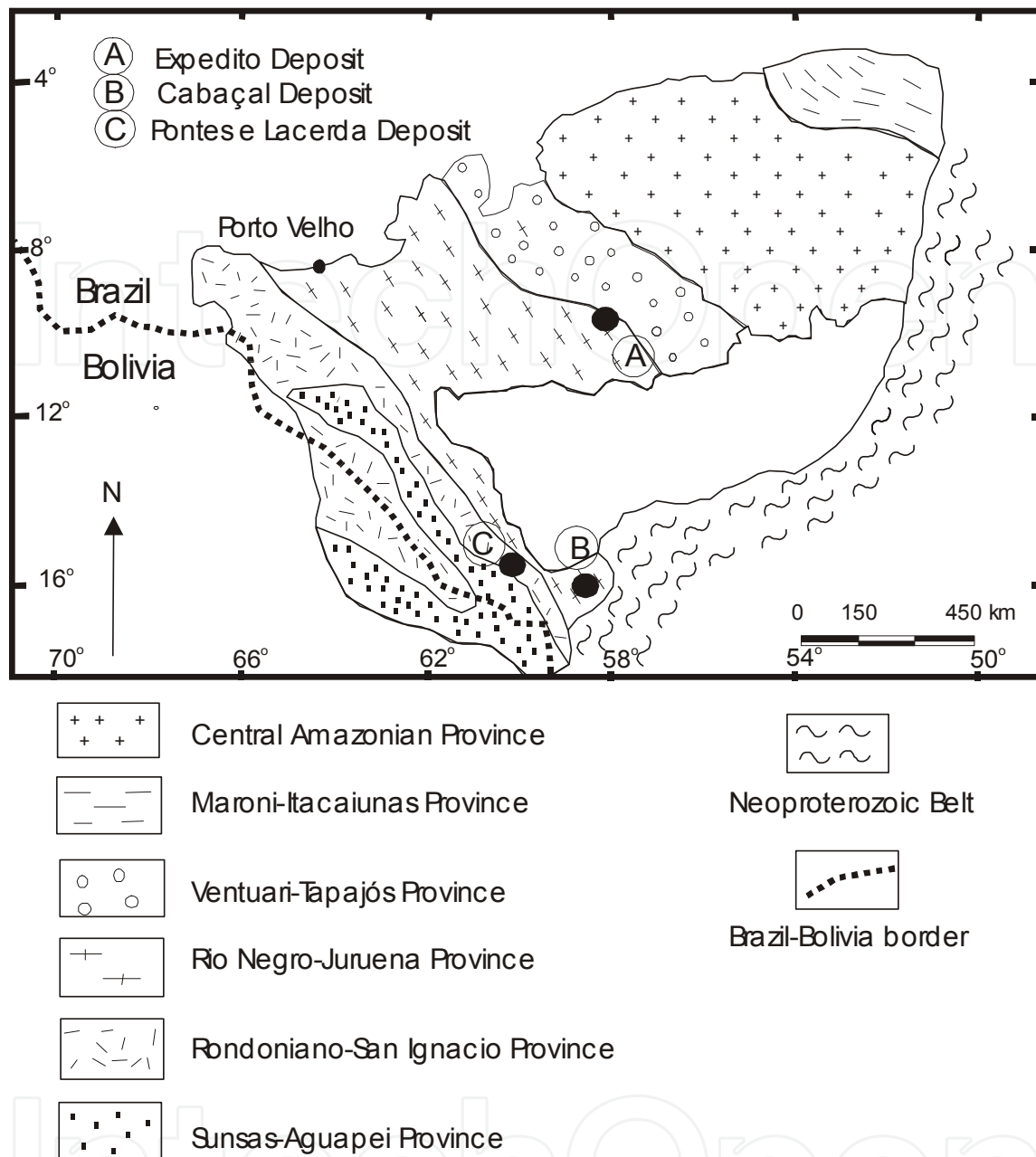
Fig. 1. Mineral deposits location and Geochronological Provinces of the southern sector of the Amazonian craton. The Cabaçal, Exedito and Pontes e Lacerda deposits are located in the map.
