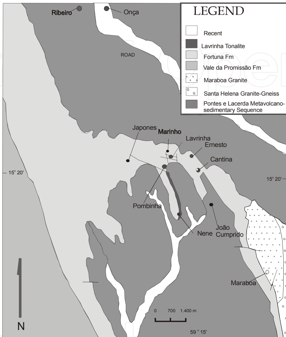
Fig. 4. Geologic map of the Pontes e Lacerda main ore deposits. Adapted from Geraldés et al. (1997).
