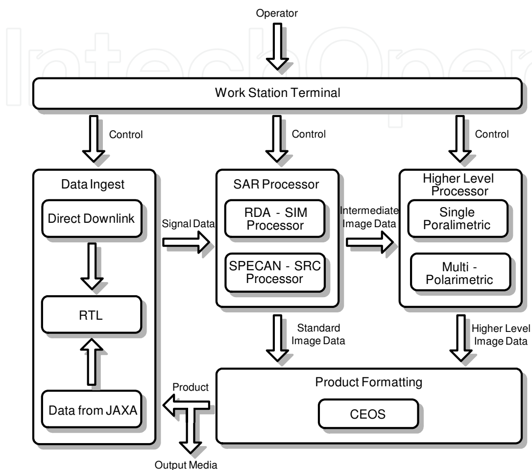
Fig. 6. ALOS SDPS Logical Architecture.
