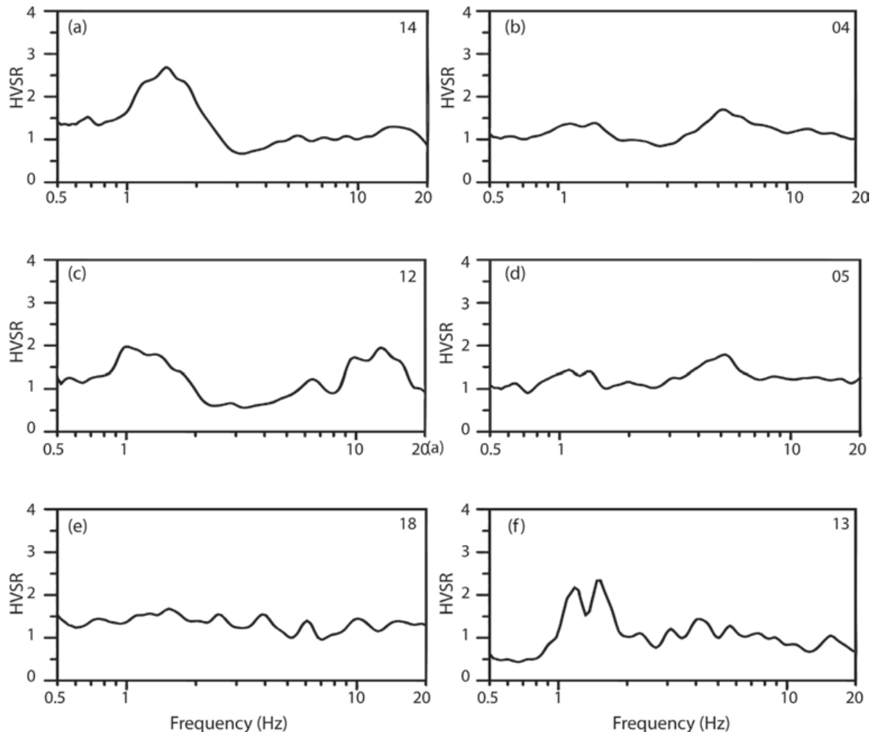
Fig. 4. Some examples of microtremor measurements for which determination of the dominant frequency may be problematic (a) wide peak, (b) two peaks, (c) artificial source of noise, (d) artificial noise which frequency can be determined, (e) almost flat spectral ratio, (f) group of peaks.
