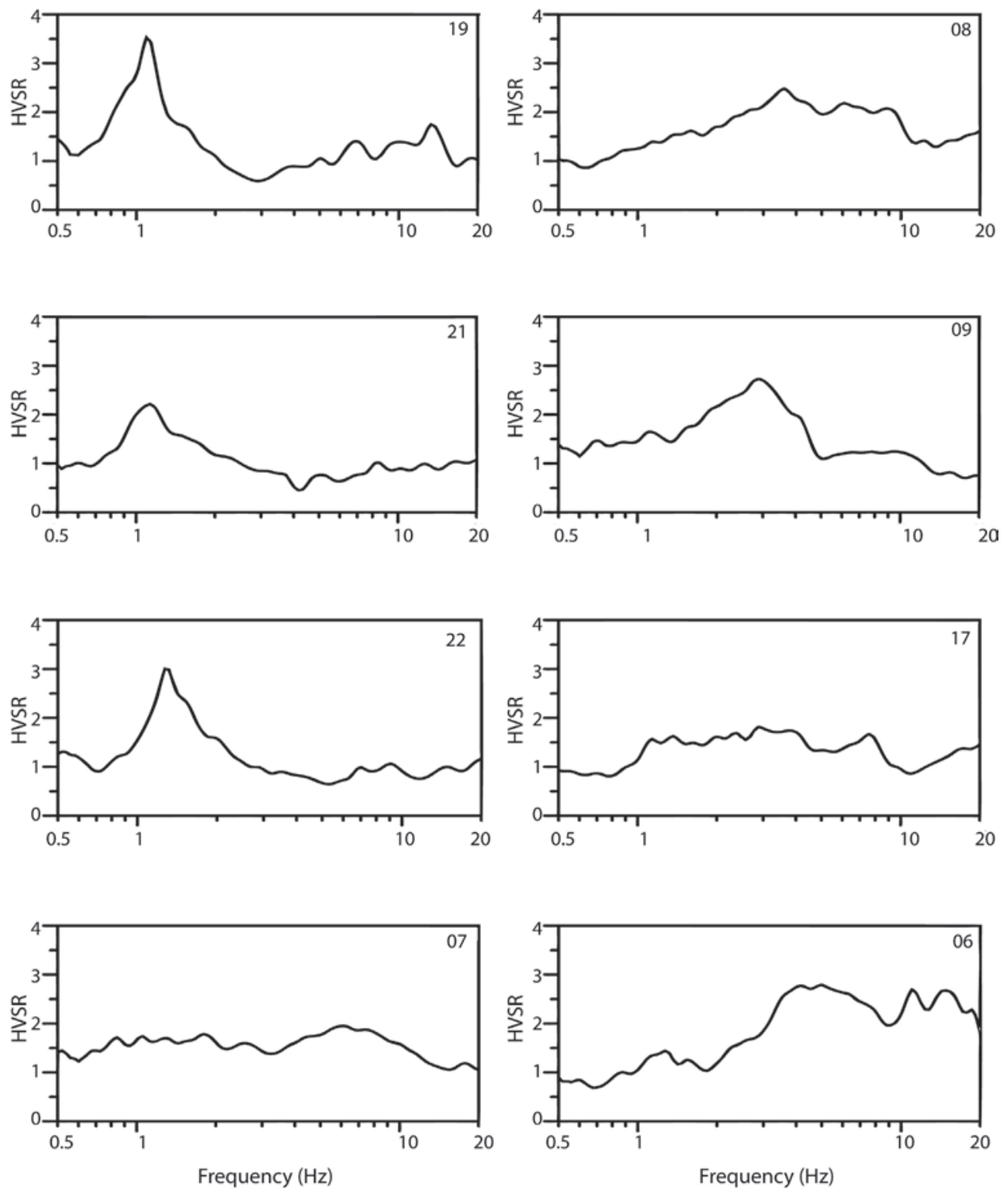
Fig. 3. Examples of HVSR for the measurements points (06, 07, 08, 09, 17, 19, 21 and 22)
