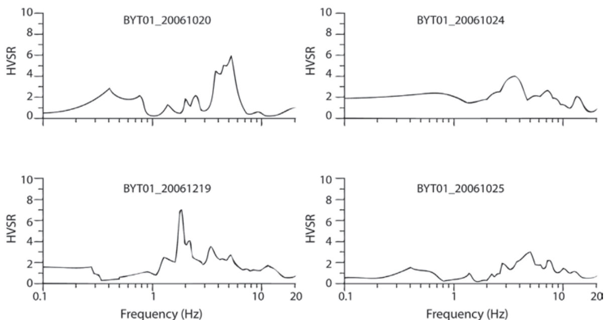
Fig. 7. The HVSR results of four earthquakes.
