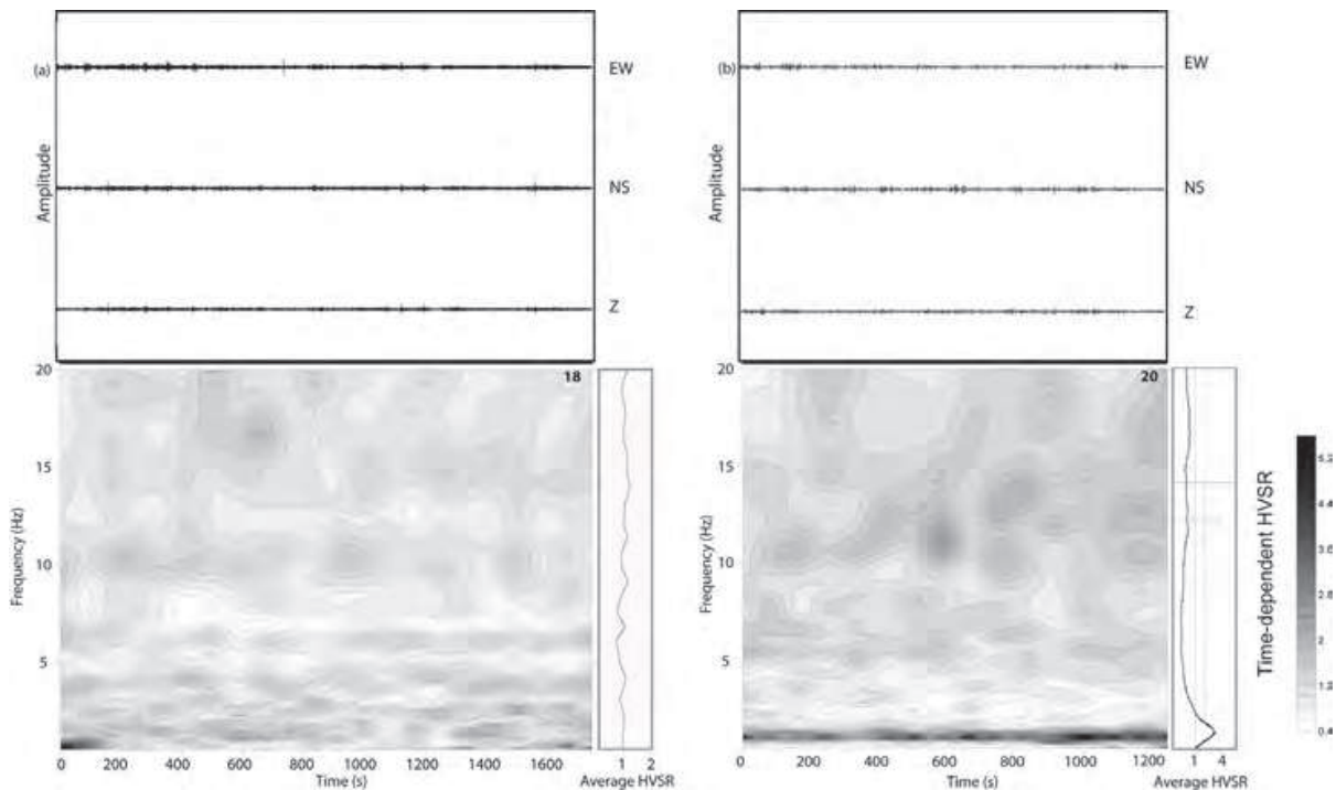
Fig. 9. Two examples of ratiograms and average HVSRs obtained from microtremors recorded at stations a) 18 and b) 20.
