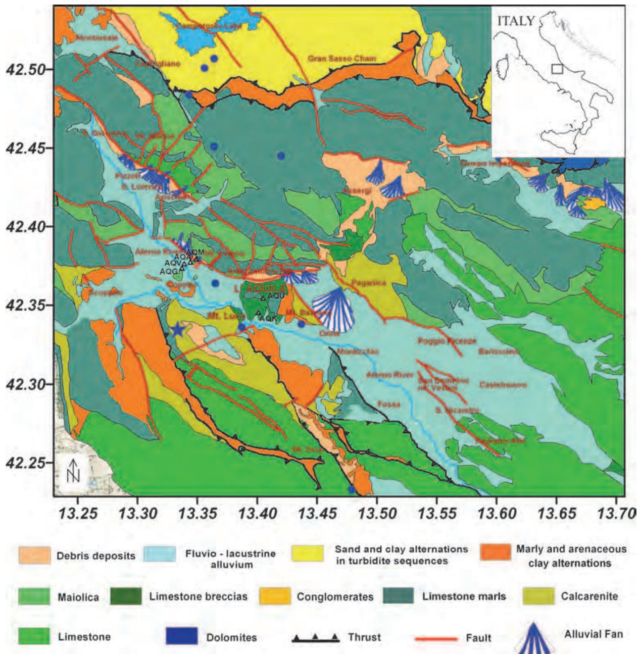
Fig. 2. Geological map of L'Aquila (modified from Vezzani and Ghisetti, 1998) with location of the RAN stations (black triangles), the main shock epicentre (blue star), the events in April 2009 (blue dots) and the site of the active seismic experiment (red square).
