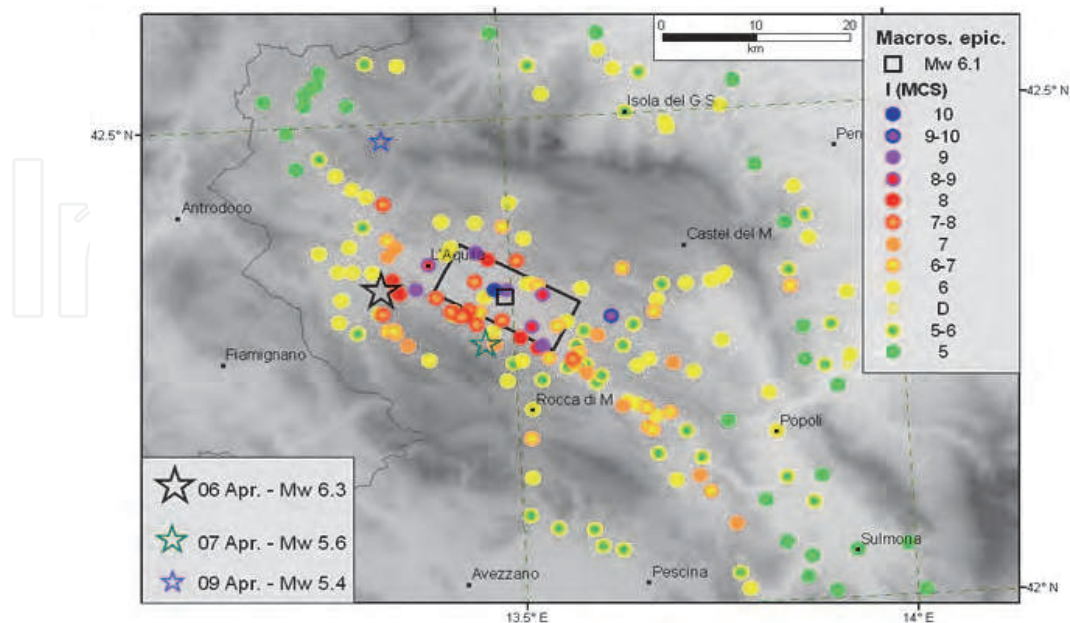
Fig. 1. Map of the effects of the 6 April 2009 earthquake and relative seismic box (from http://www.mi.ingv.it/eq/090406/quest.html )
