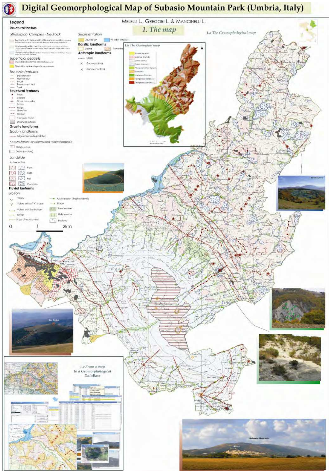
Fig. 10. The final layout of the geomorphological map (front side) with the geomorphological map, a geological sketch, some significant photos and the scheme of the transition from the analogical product to the digital one.
