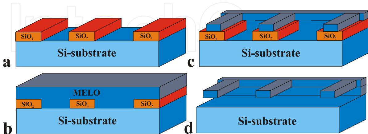
Fig. 11. Basic MELO process.
