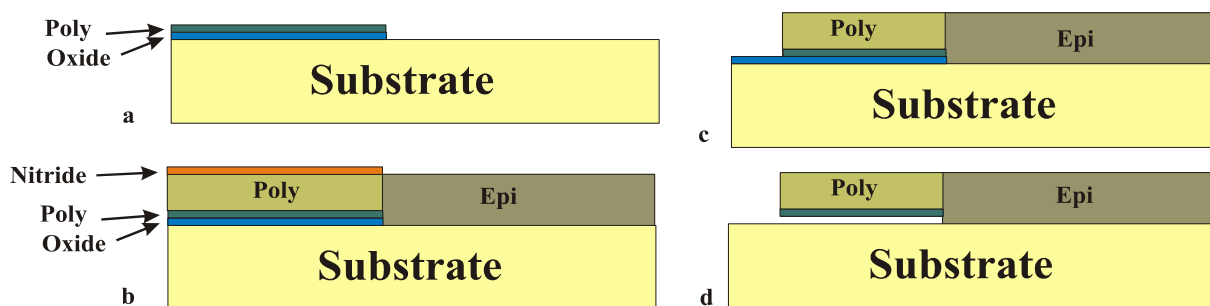
Fig. 13. Basic epi-poly process.
