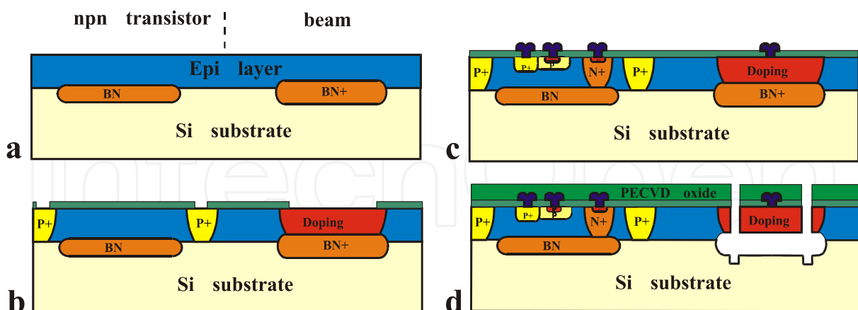
Fig. 7. Main steps for the SIMPLE process.
