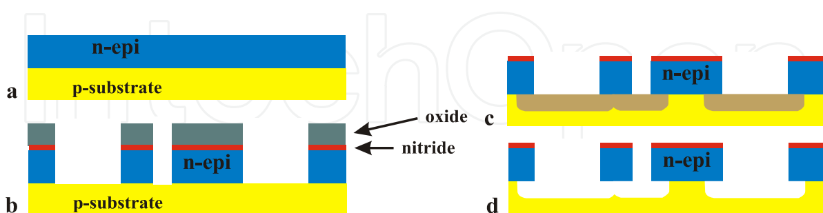
Fig. 12. Basic process steps for sacrificial porous silicon based micromachining
