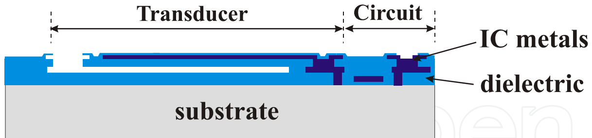
Fig. 21. Micromachining integrated into a CMOS process
