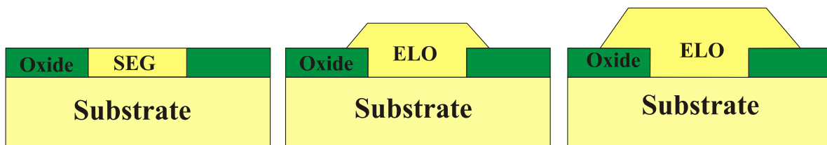
Fig. 10. Basic SEG process extended to ELO
